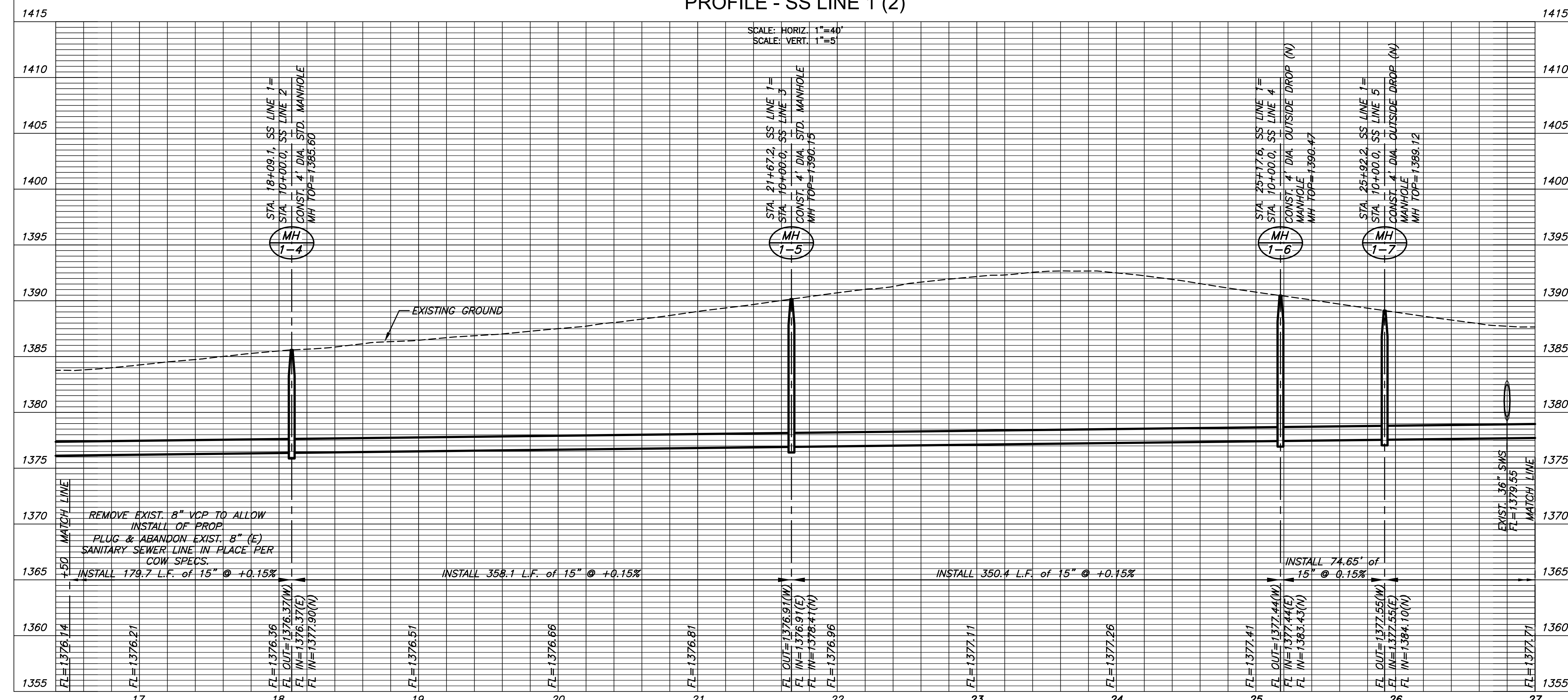
PLAN - SS LINE 1 (2) PROFILE - SS LINE 1 (2)
