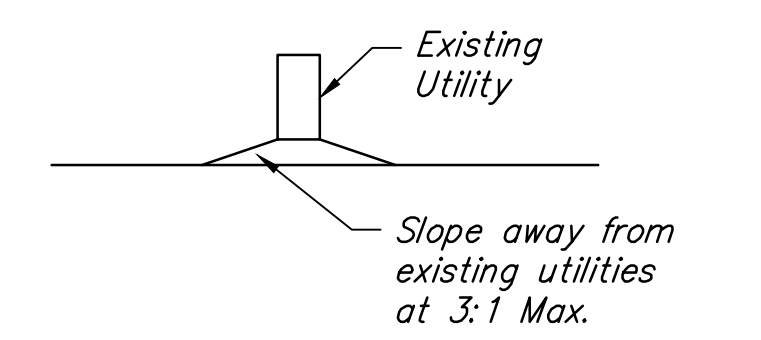
GRADING AT EXISTING UTILITIES
