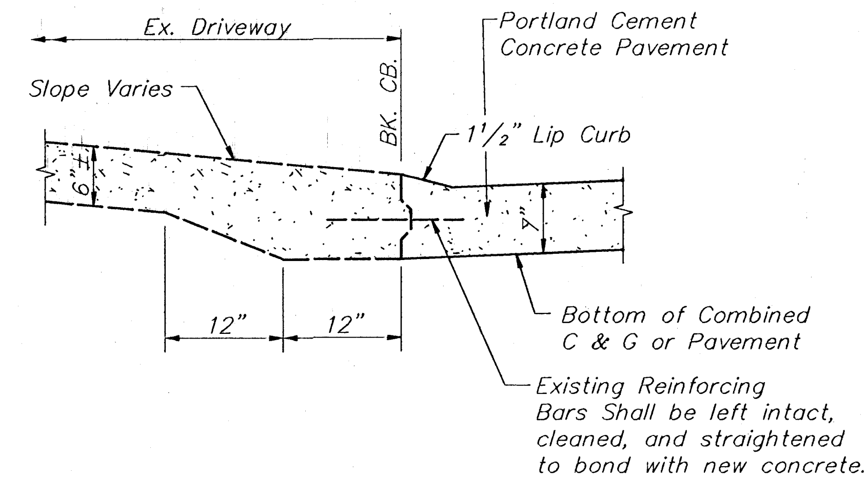
SECTION A-A BACK OF CURB DETAIL Not To Scale
