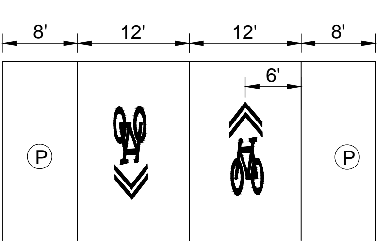
PROPOSED MARKET STREET E. 20TH STREET TO E. 21ST STREET
