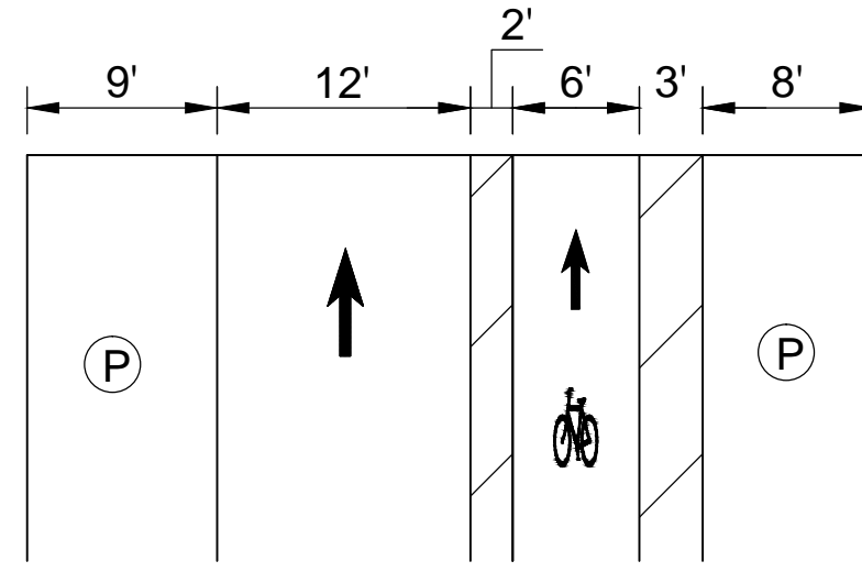
PROPOSED MARKET STREET E. 11TH STREET TO E. 12TH STREET
