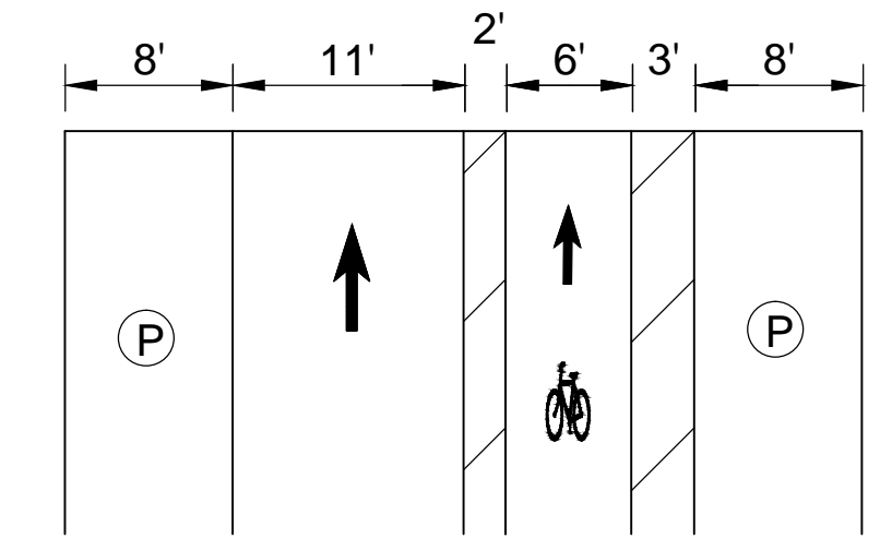
PROPOSED MARKET STREET E. 15TH STREET TO E. 16TH STREET
