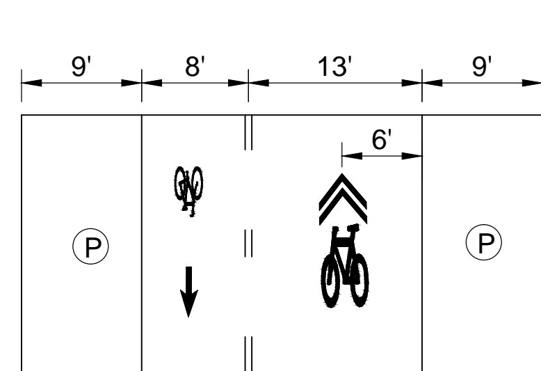
PROPOSED MARKET STREET E. 19TH STREET TO E. 20TH STREET
