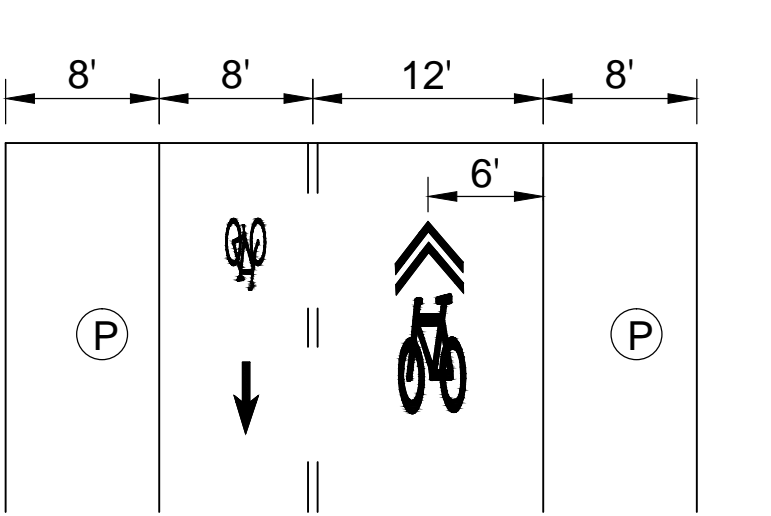
PROPOSED MARKET STREET E. 17TH STREET TO E. 18TH STREET
