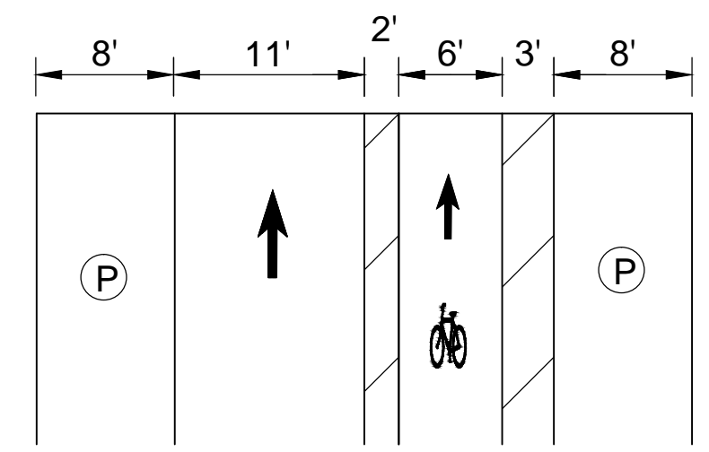
PROPOSED MARKET STREET E. 14TH STREET TO E. 15TH STREET
