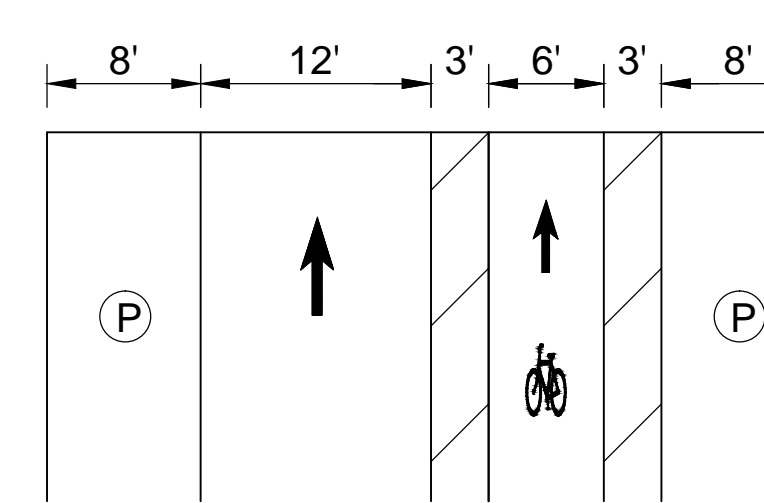
PROPOSED MARKET STREET E. 12TH STREET TO E. 13TH STREET
