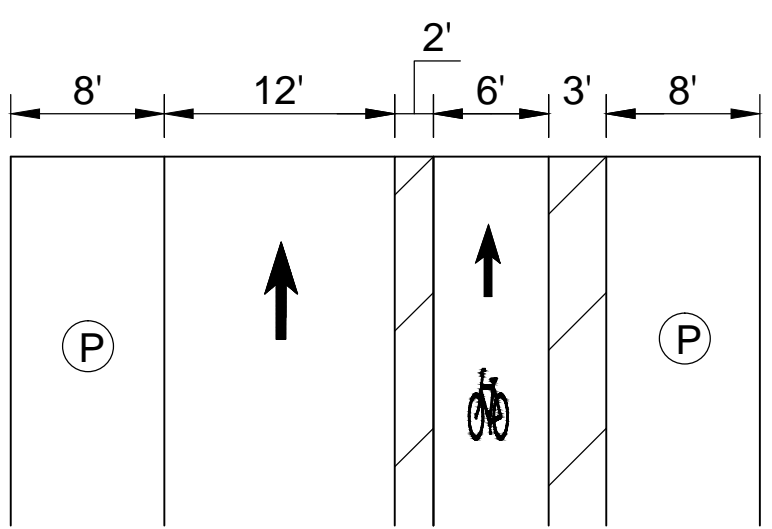
PROPOSED MARKET STREET E. 13TH STREET TO E. 14TH STREET
