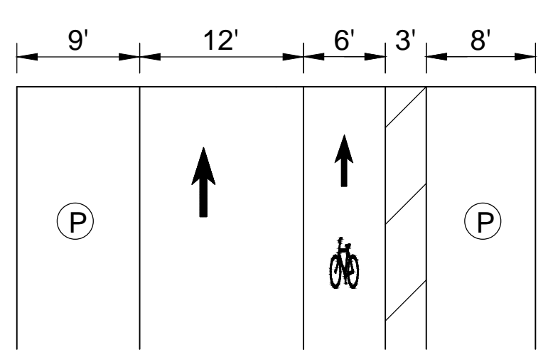
PROPOSED MARKET STREET E. 16TH STREET TO E. 17TH STREET
