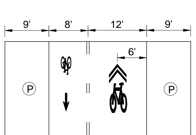
PROPOSED MARKET STREET E. 18TH STREET TO E. 19TH STREET
