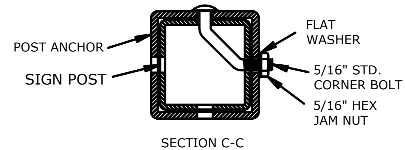
DETAILS FOR 2 1/2" SIGN POST
