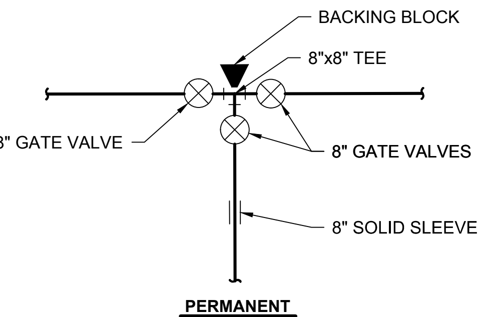
CONNECTION DETAIL NOT TO SCALE
