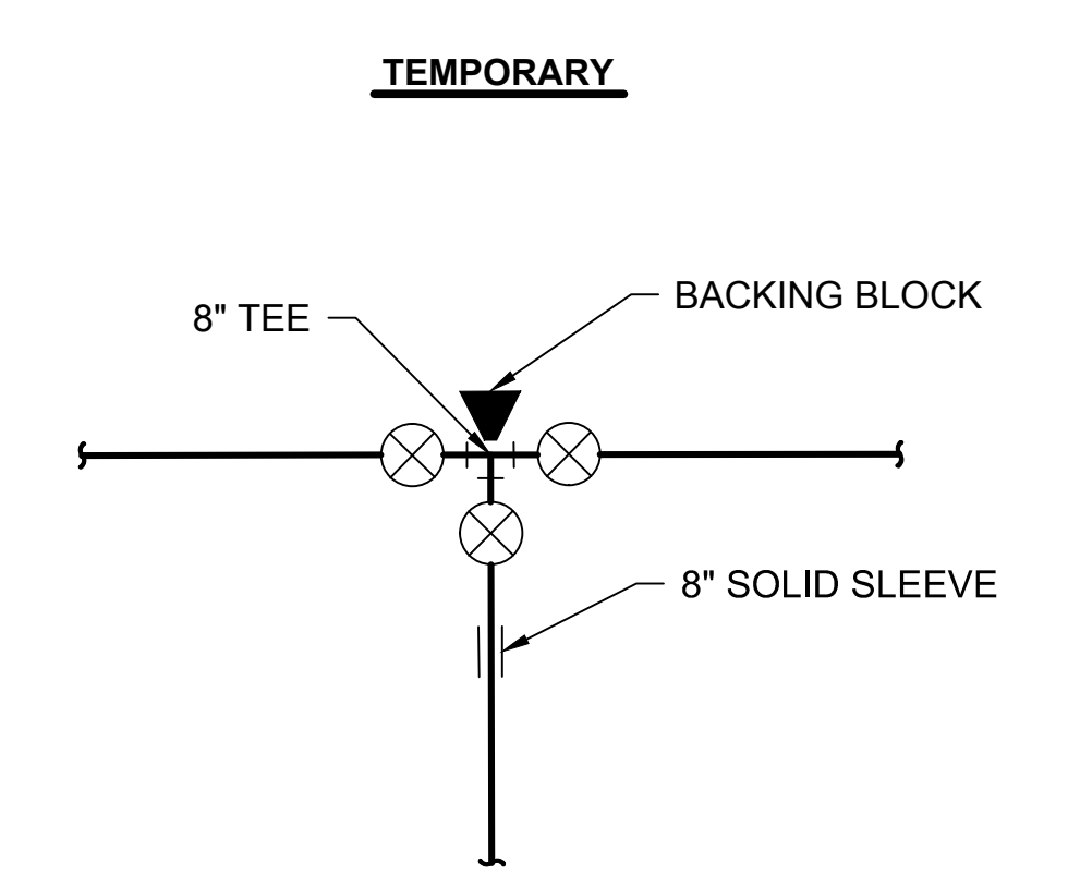
CONNECTION DETAIL NOT TO SCALE
