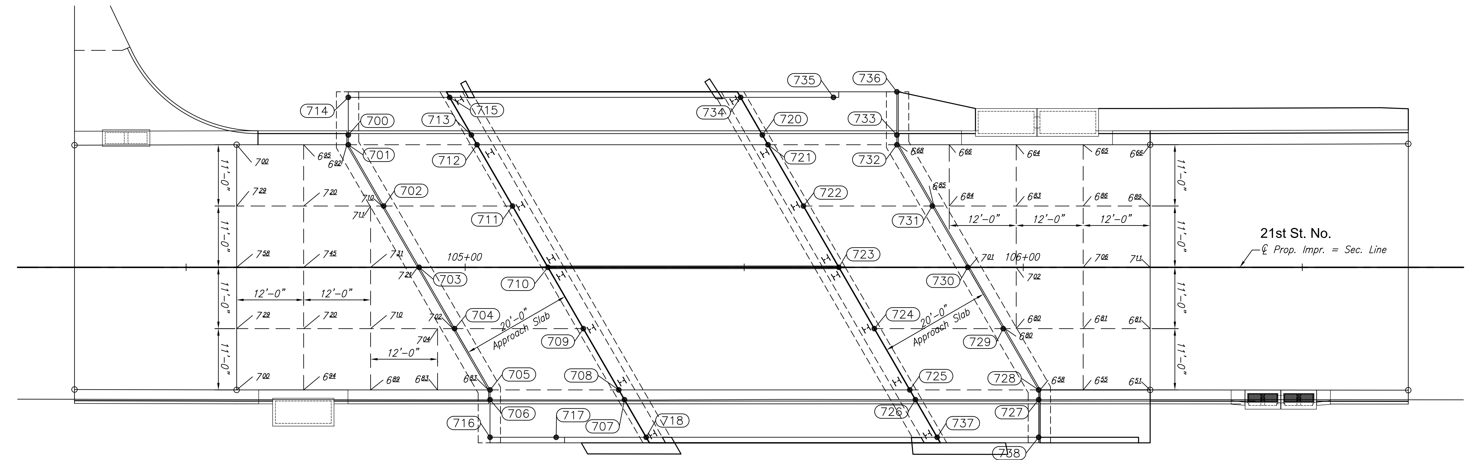
APPROACH SLAB ELEVATION PLAN
