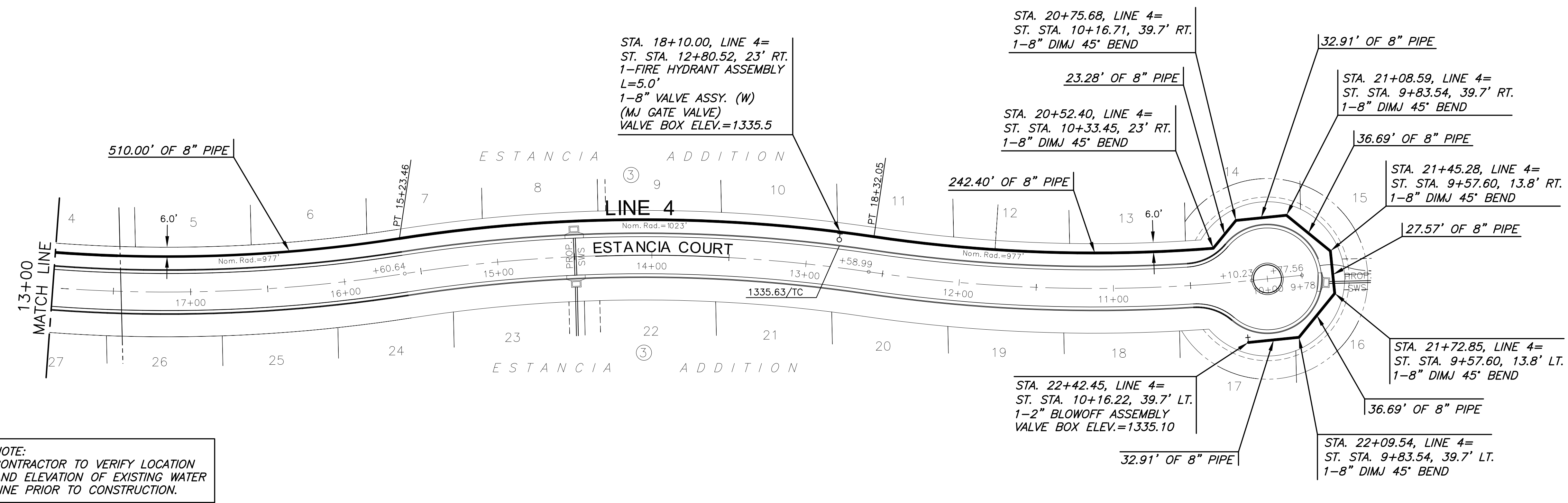
PLAN LINE 4 PROFILE LINE 4
