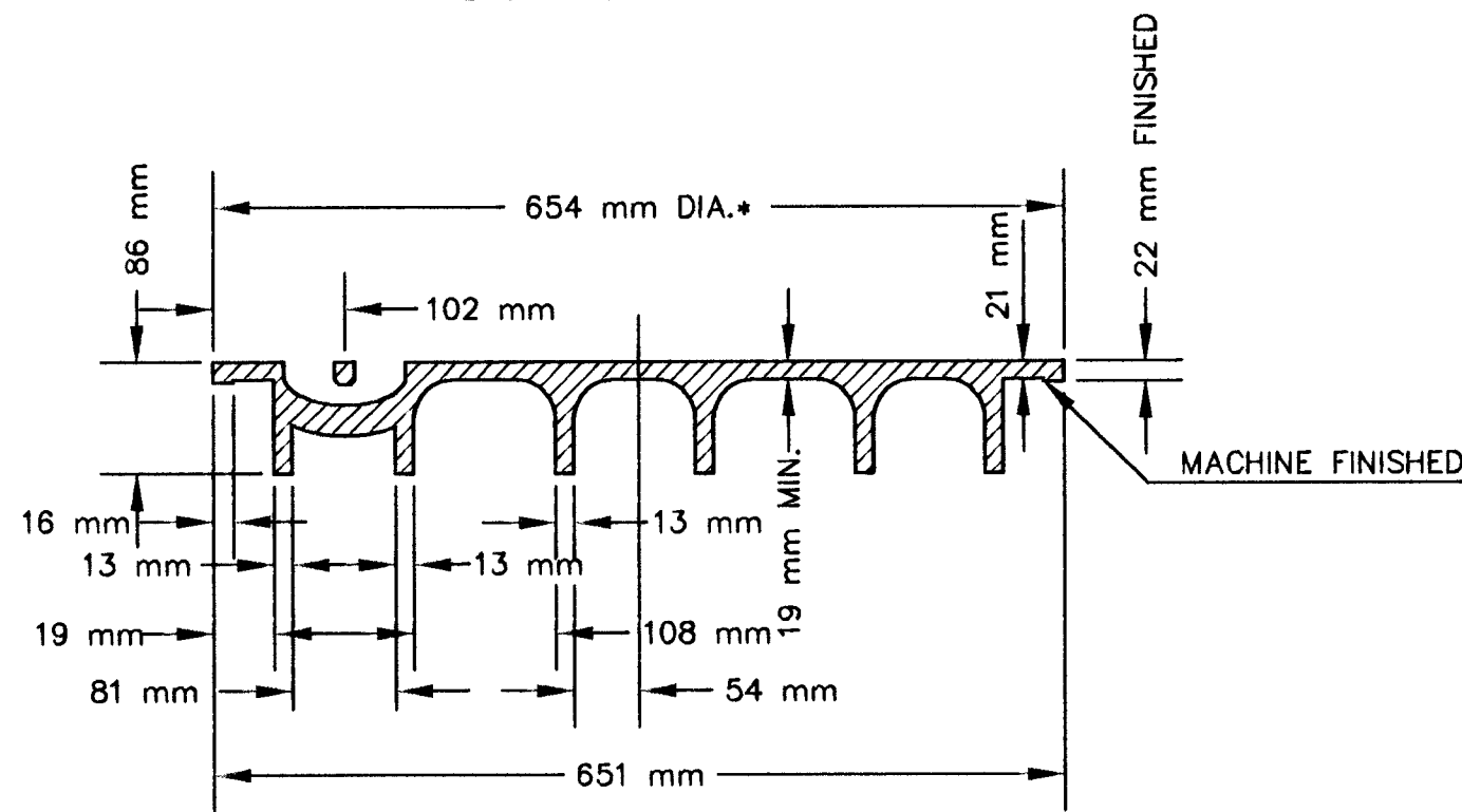
BOTTOM VIEW
