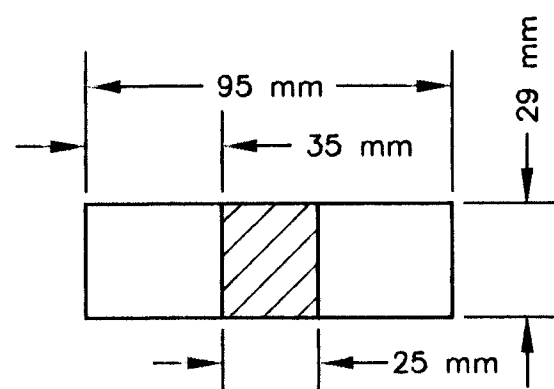
PICKHOLE DETAIL
