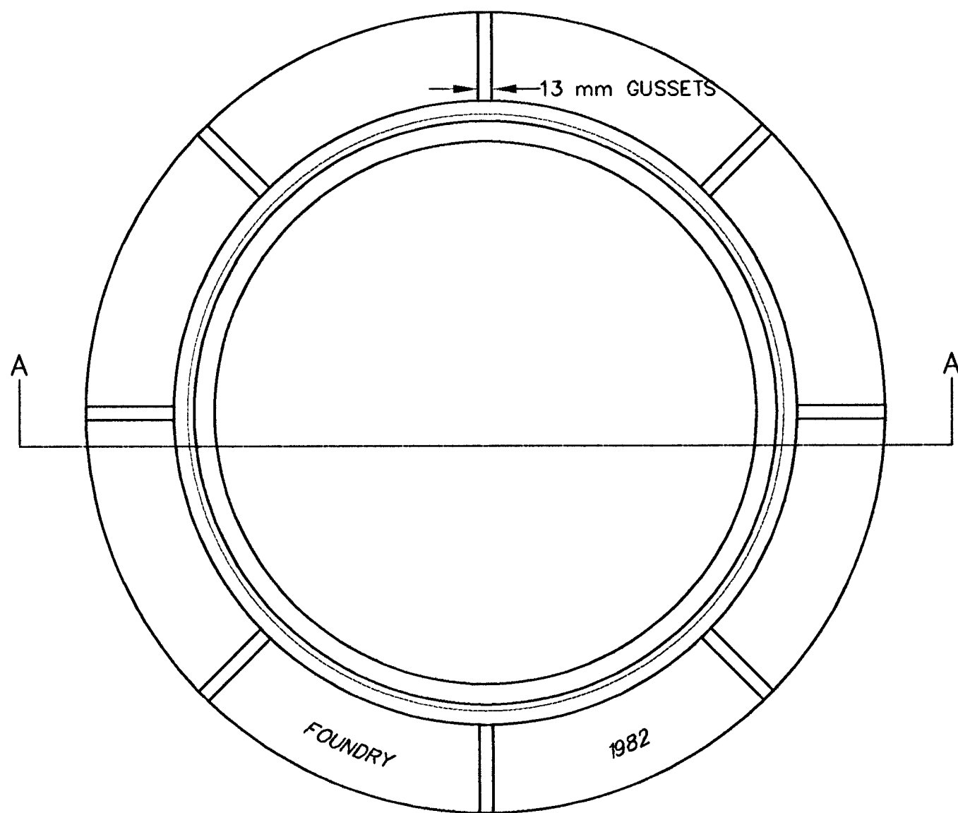
MANHOLE FRAME WEIGHT: 108.844 kg
