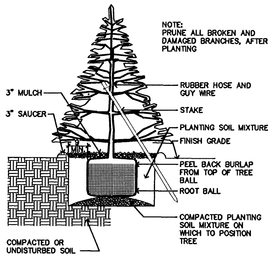
1 EVERGREEN TREE PLANTING DETAIL NOT TO SCALE
