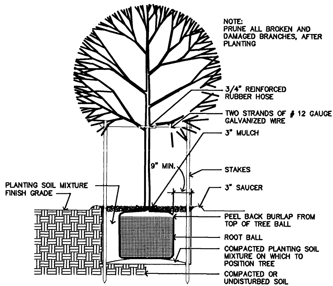
2 DECIDUOUS TREE PLANTING DETAIL NOT TO SCALE
