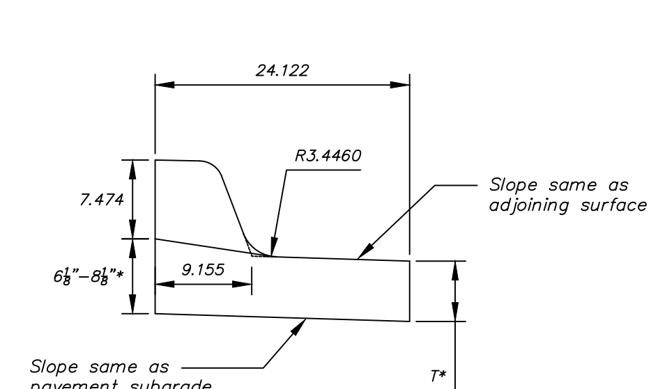
Combined Curb & Gutter (1 1/2")
