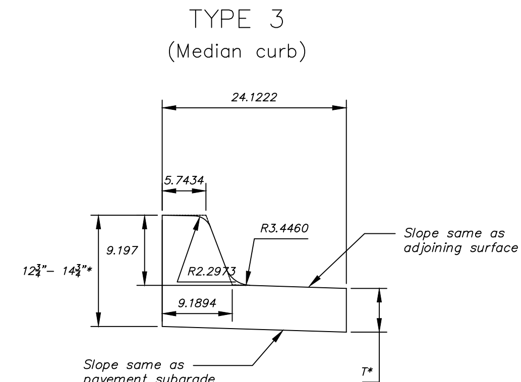
Combined Curb & Gutter (8")
