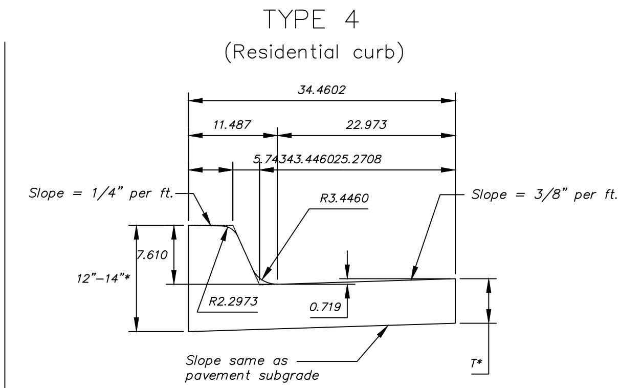
Combined Curb & Gutter (6 5/8")
