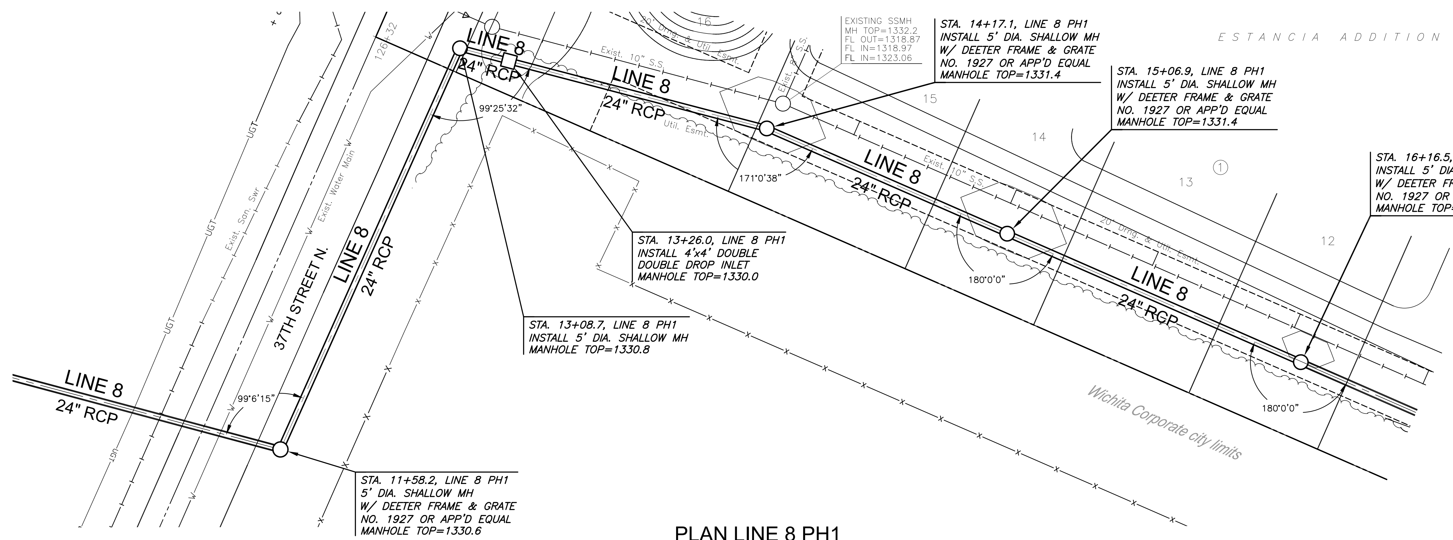
PLAN LINE 8 PH1 PROFILE LINE 8 PH1
