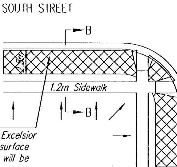
BACK OF CURB PROTECTION DETAIL
