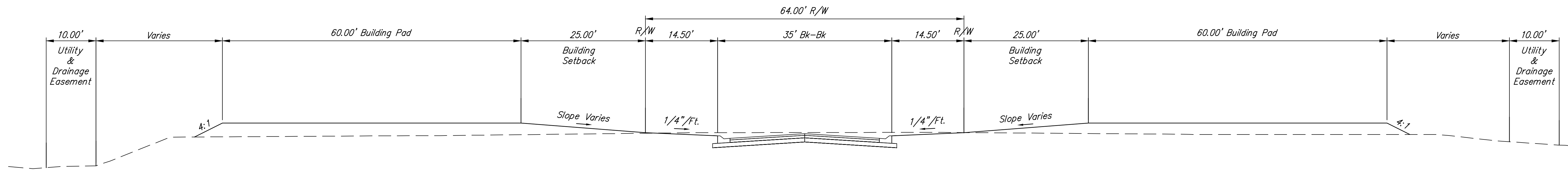
TYPICAL GRADING SECTION
