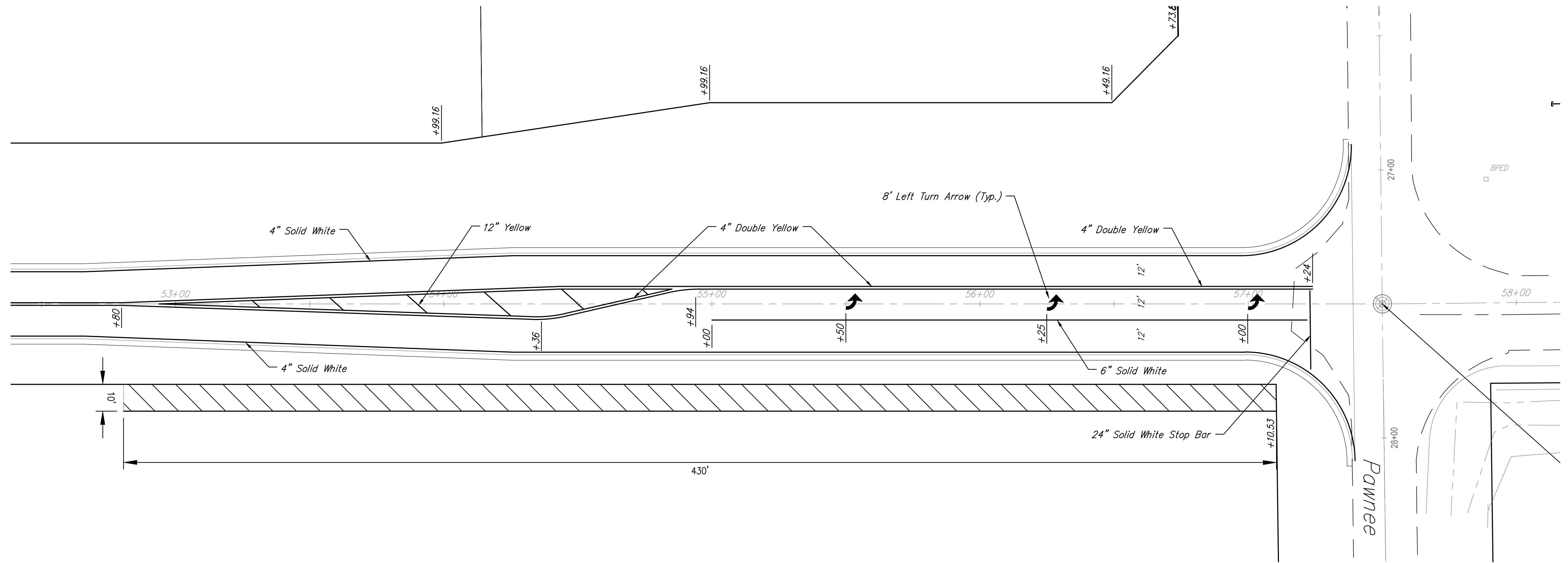
Left Turn Pavement Marking
