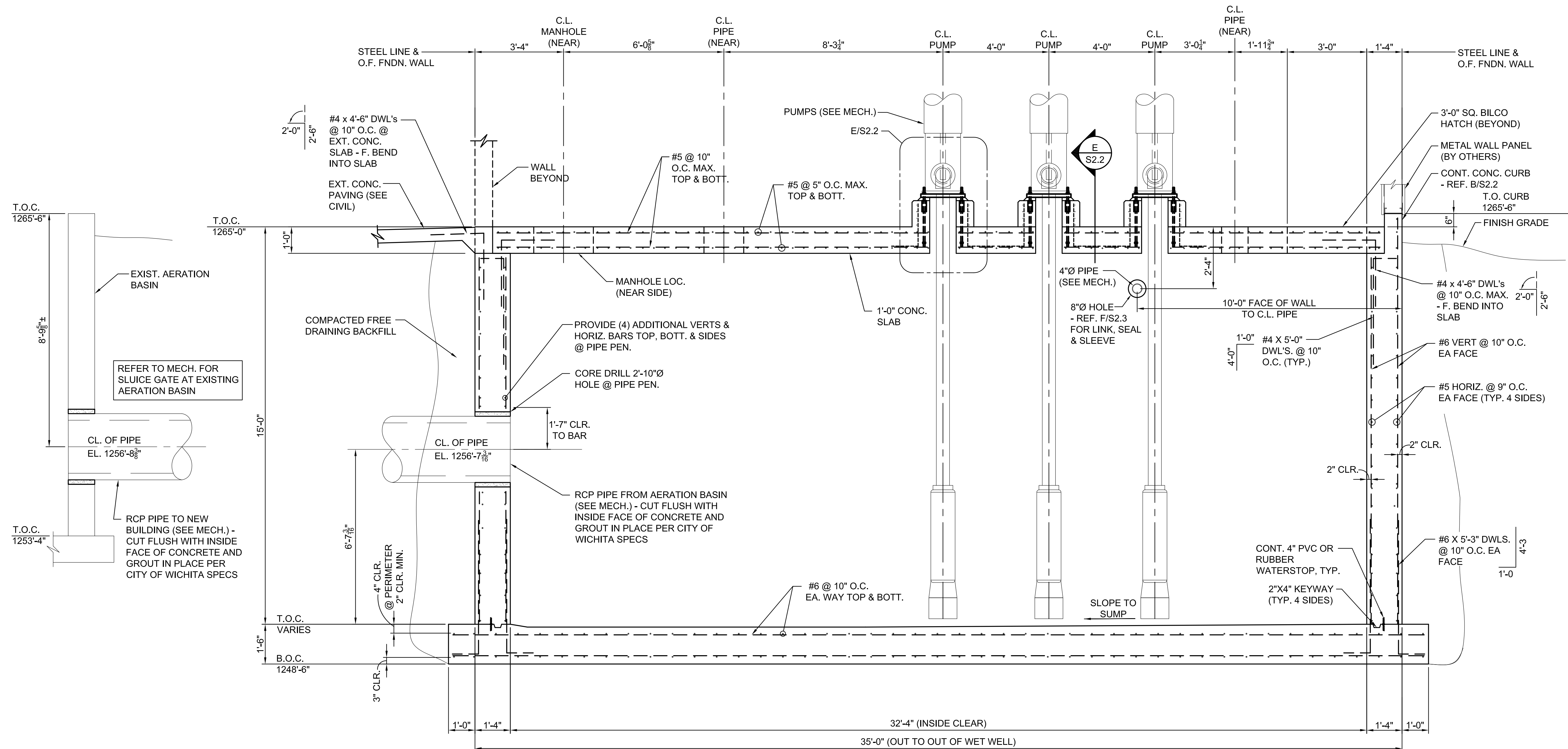
FOUNDATION SECTION SCALE: 1/2" = 1'-0"
