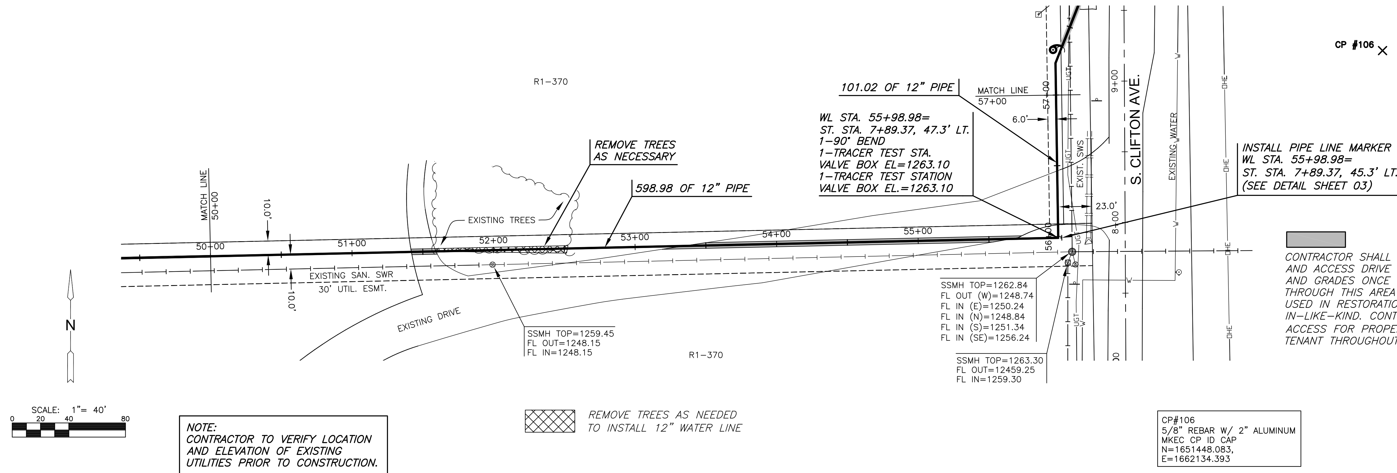
PLAN SPIRIT RE-USE LINE 50+00 - 57+00 PROFILE SPIRIT RE-USE LINE 50+00 - 57+00
