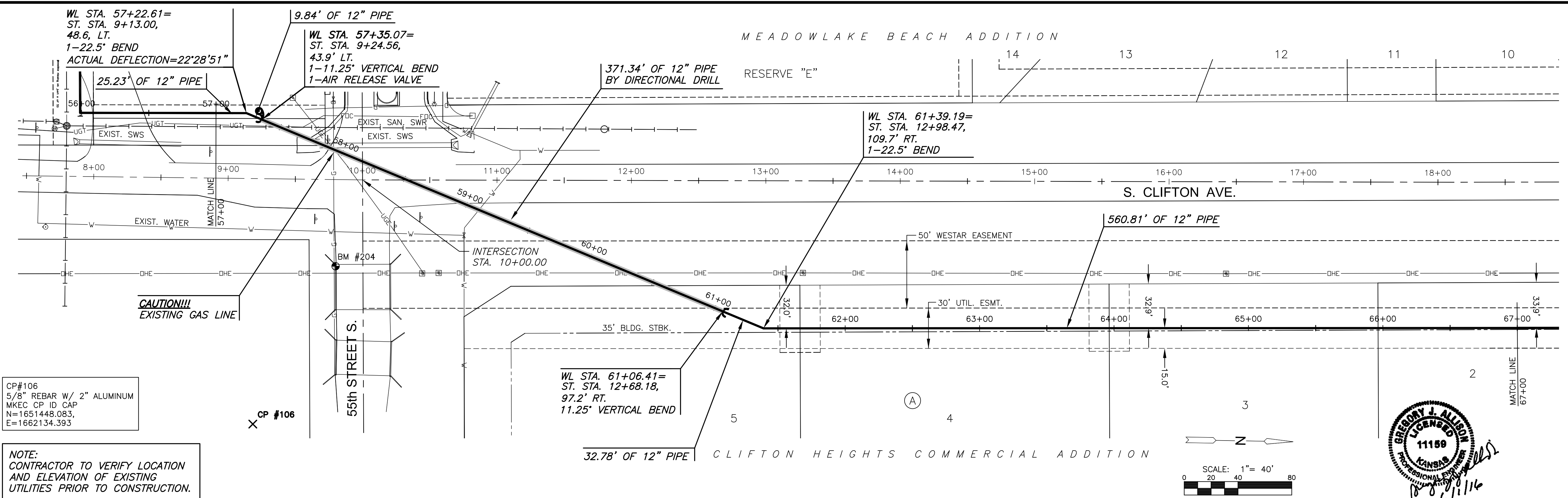
PLAN SPIRIT RE-USE LINE 57+00 - 67+00 PROFILE SPIRIT RE-USE LINE 57+00 - 67+00
