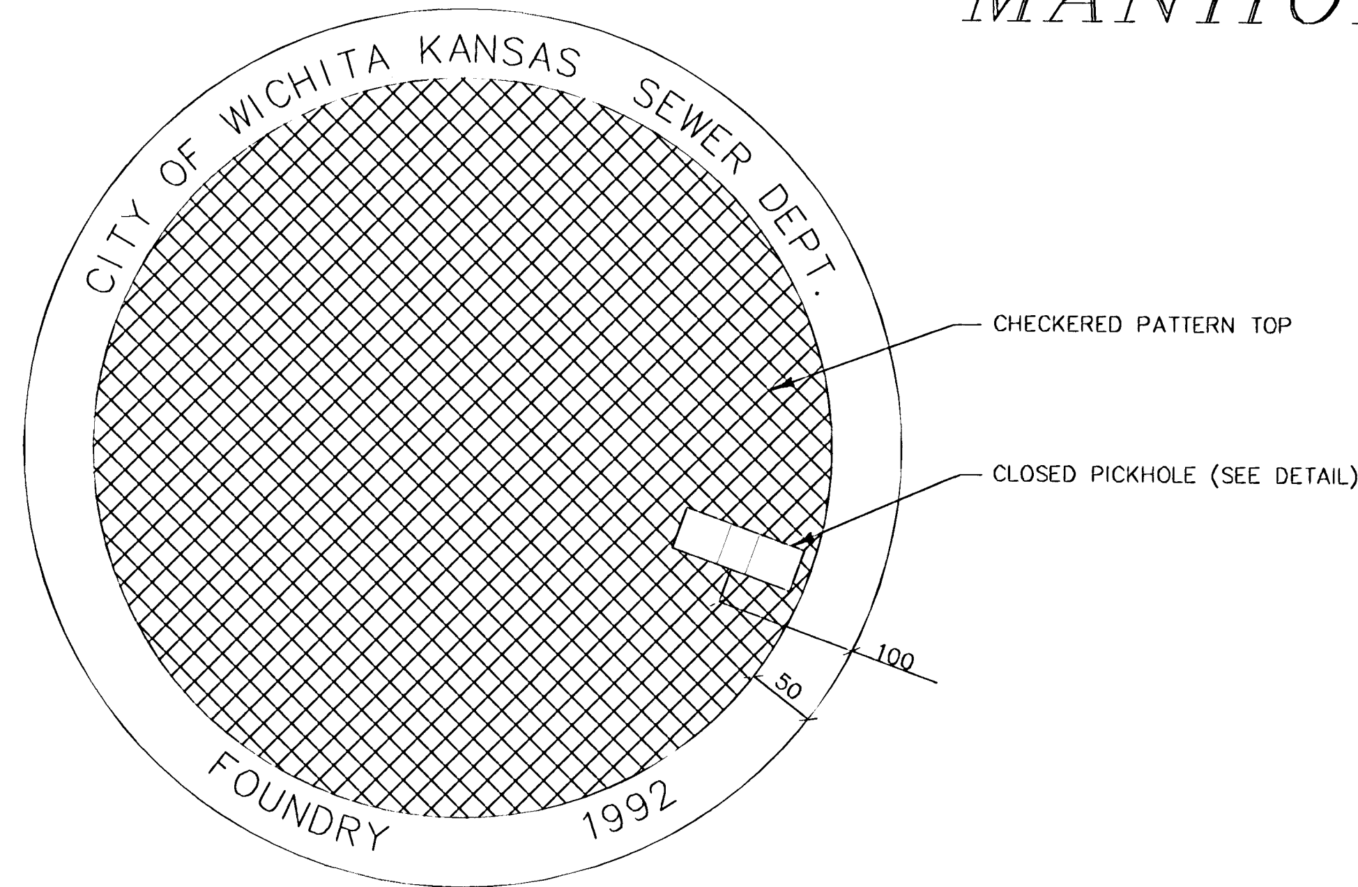
TOP VIEW
