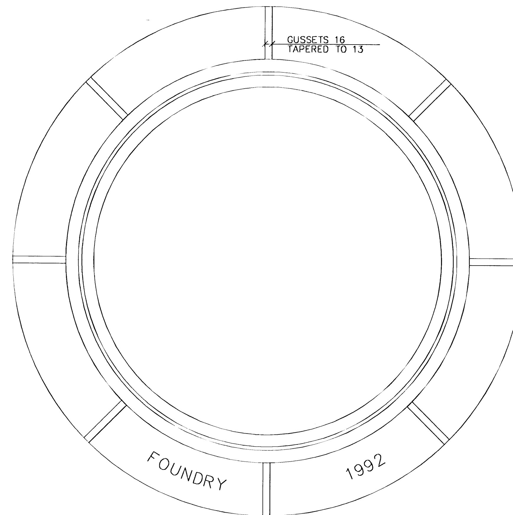
TOP VIEW
