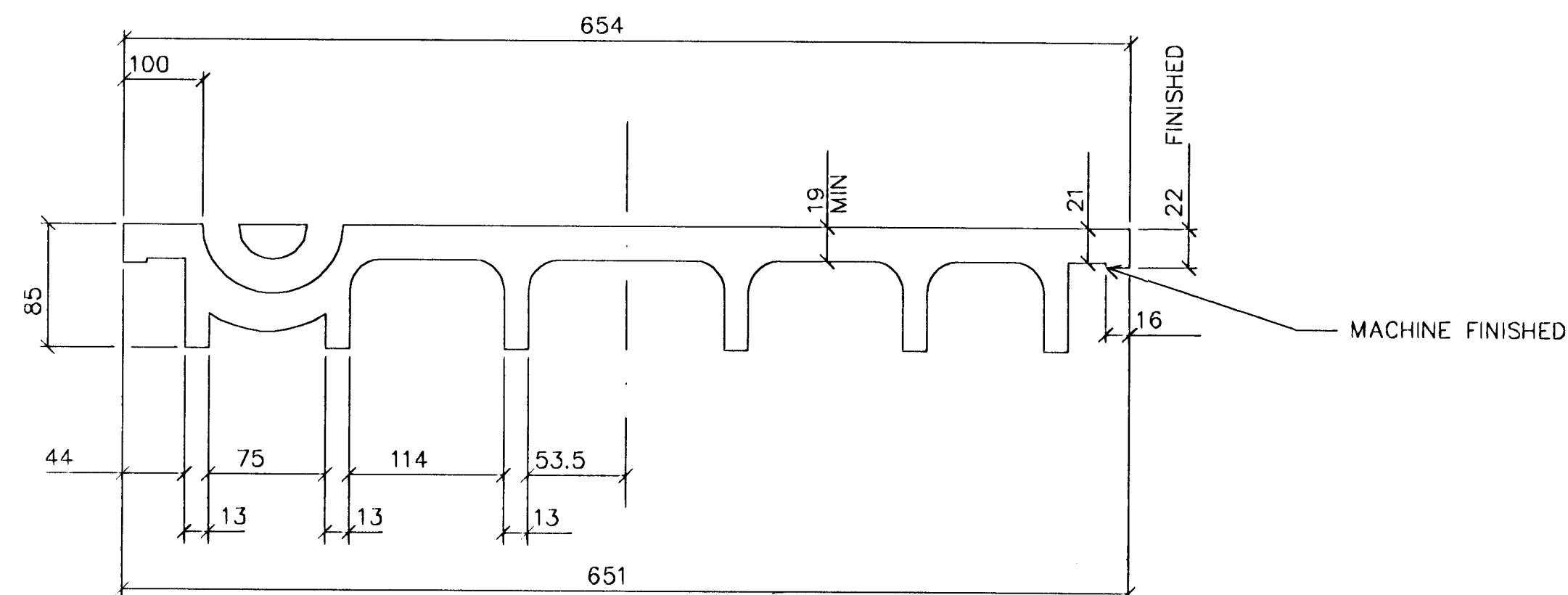
BOTTOM VIEW
