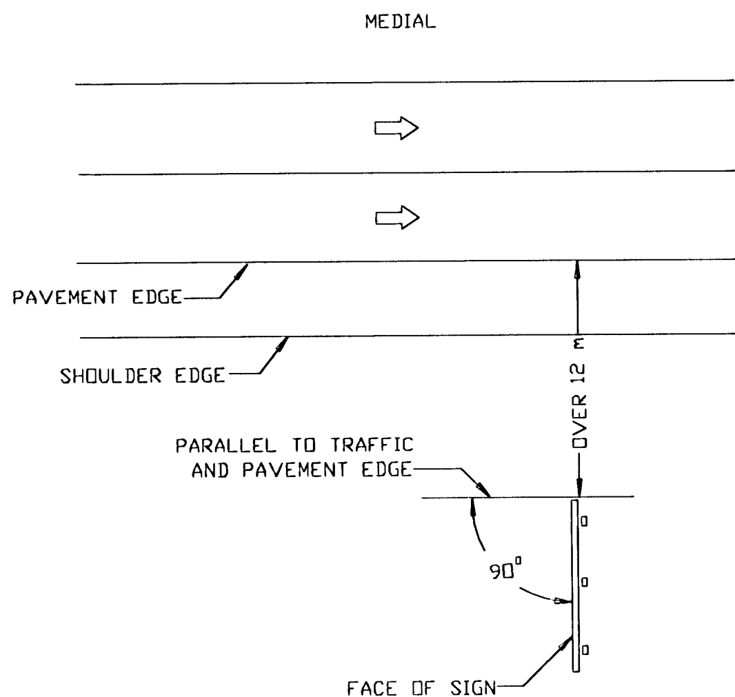
ANGLE OF REFLECTORIZED SIGN ERRECTED OVER 12 m OUT FROM THE PAVEMENT EDGE ON STRAIGHT ROADWAY
