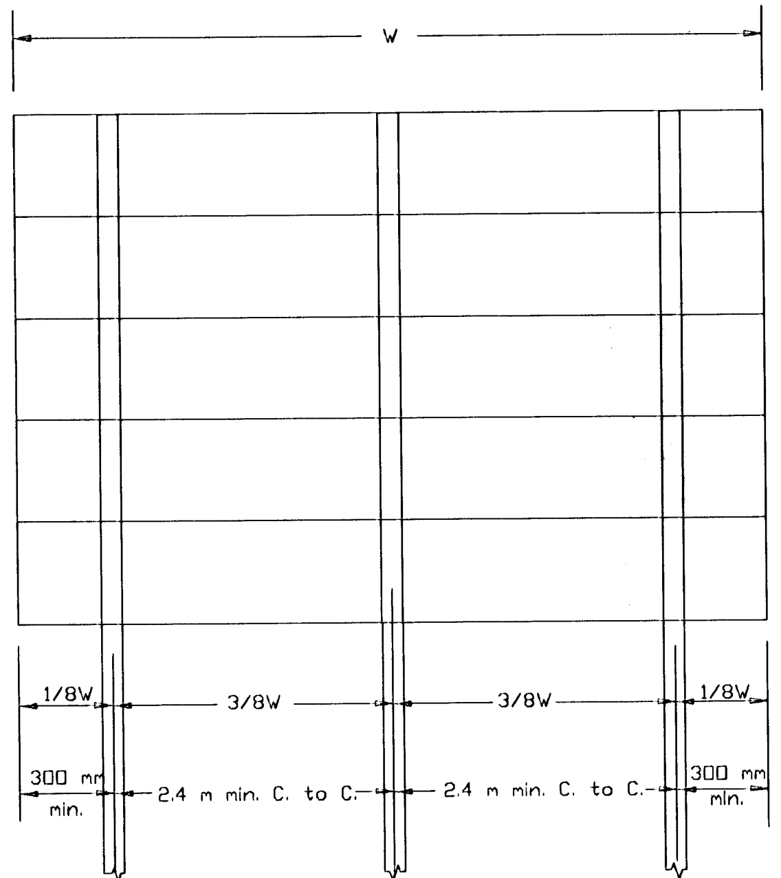
THREE POST SPACING
