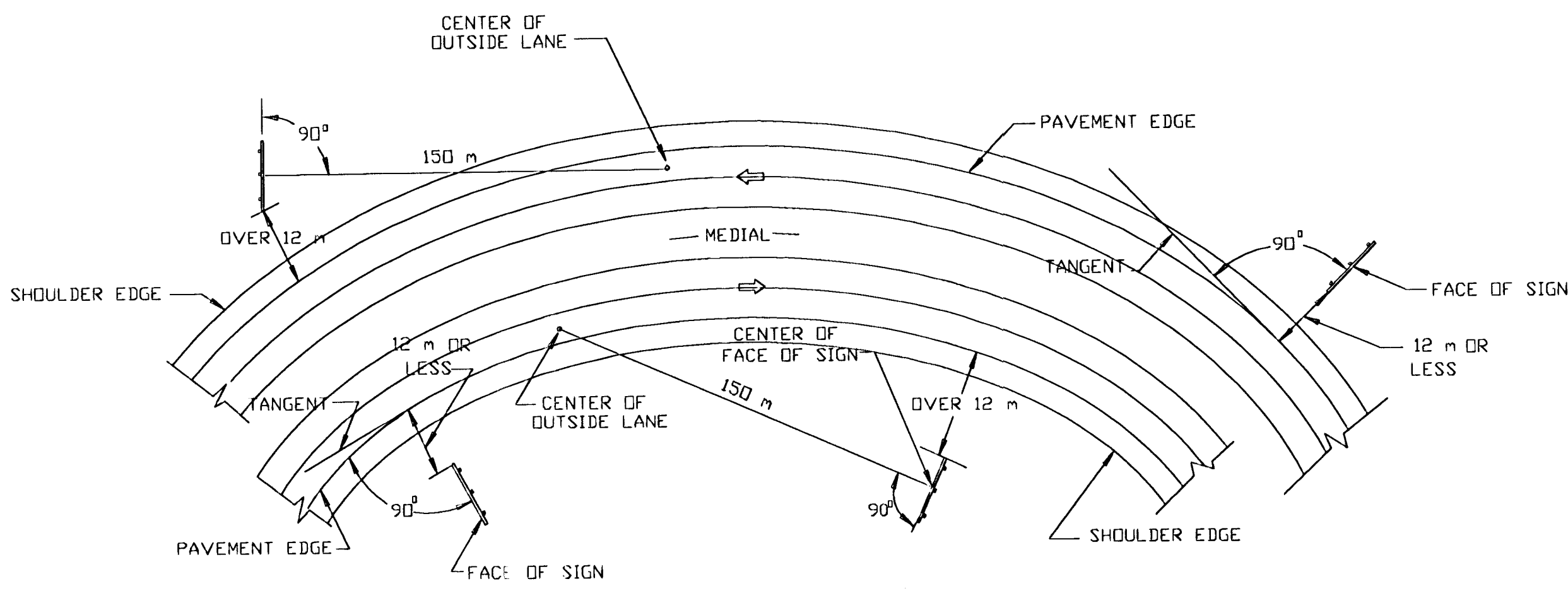
ANGLE OF REFLECTORIZED SIGNS ERRECTED 12 m OR LESS OUT FROM THE PAVEMENT EDGE AND OVER 40' OUT FROM PAVEMENT EDGE ON CURVED ROADWAY
