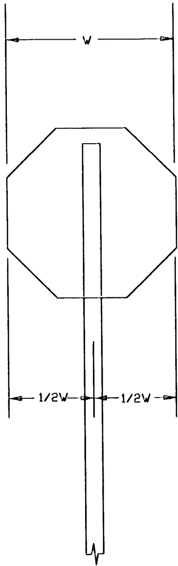
ONE POST SPACING
