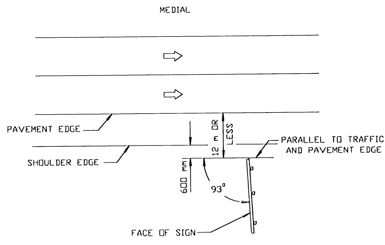
ANGLE OF REFLECTORIZED SIGN ERRECTED 12 m OR LESS OUT FROM THE PAVEMENT EDGE
