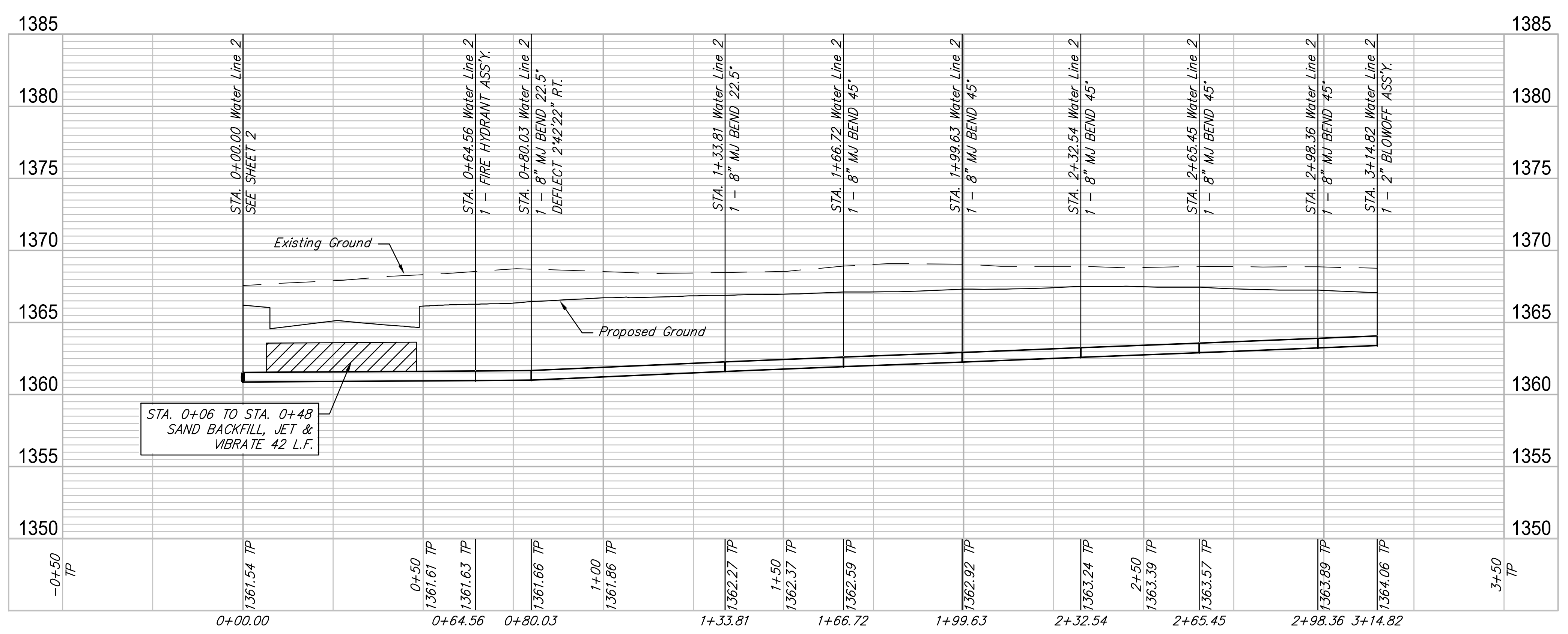
Water Line 2 PROFILE
