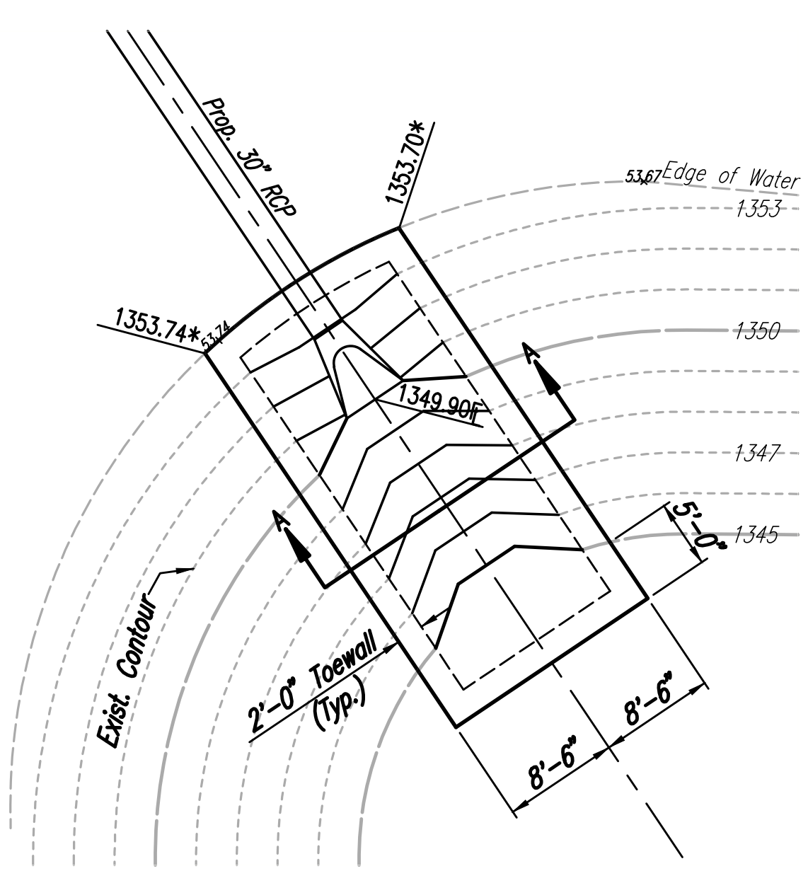
RIPRAP PLAN (SWS Line No. 1)
