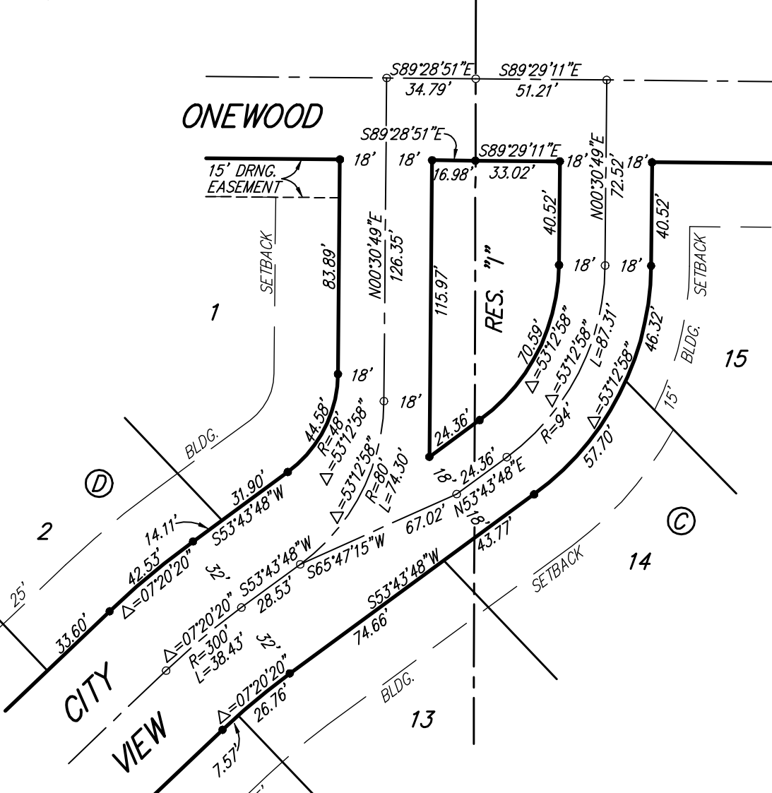
DETAIL "B" (NO SCALE)
