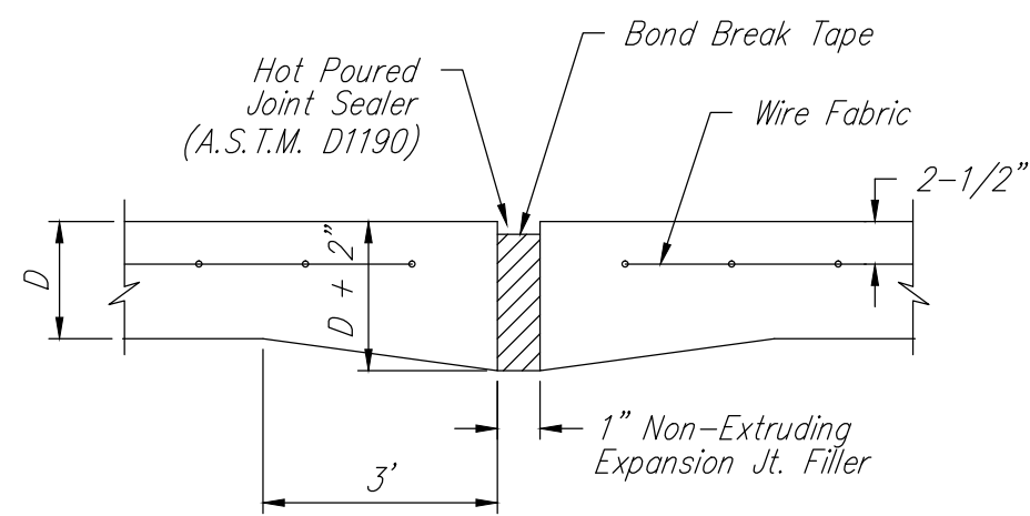
EXPANSION JOINT (E.J.)
