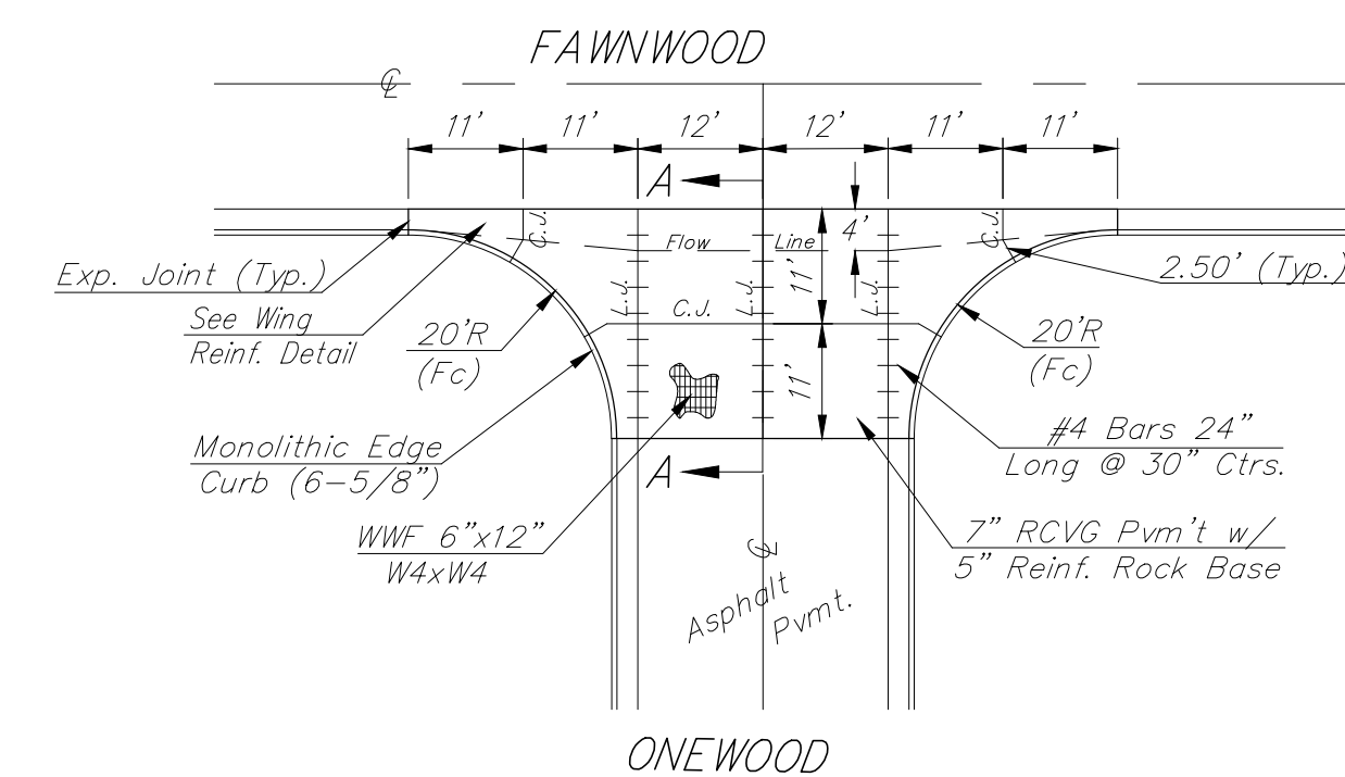
REINFORCED VALLEY GUTTER DETAIL
