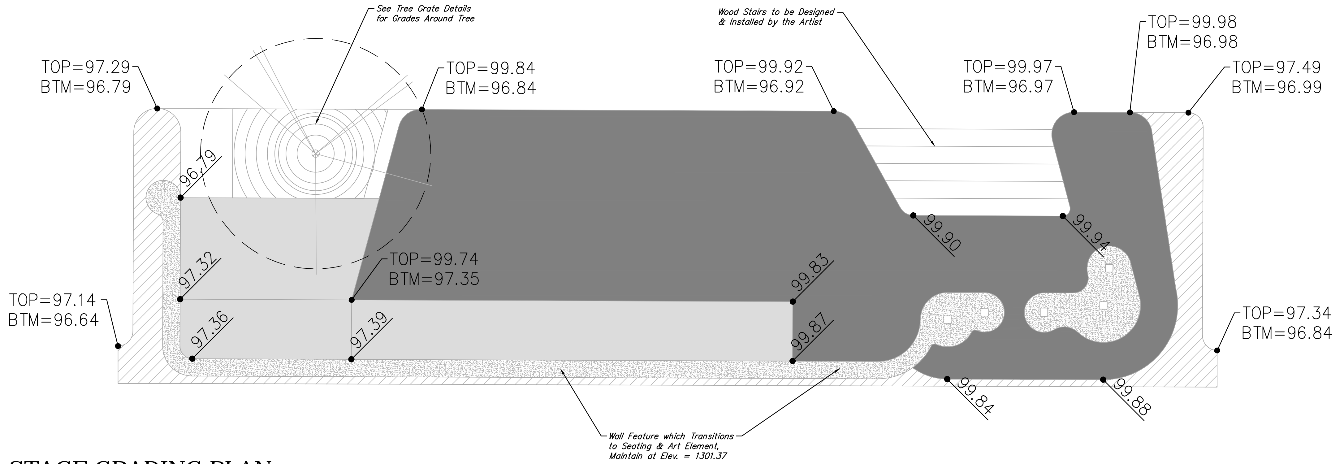
STAGE GRADING PLAN 1"=4'
