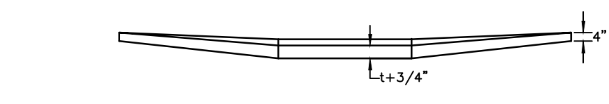
SECTION B-B
