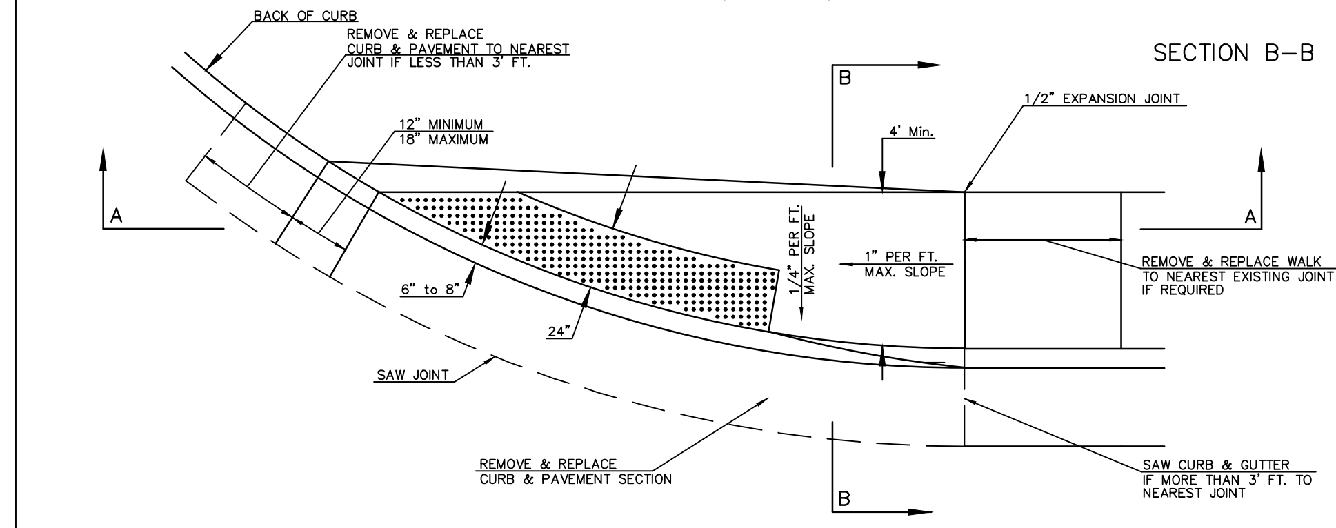
SECTION B-B
