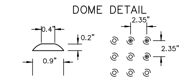
DOME DETAIL
