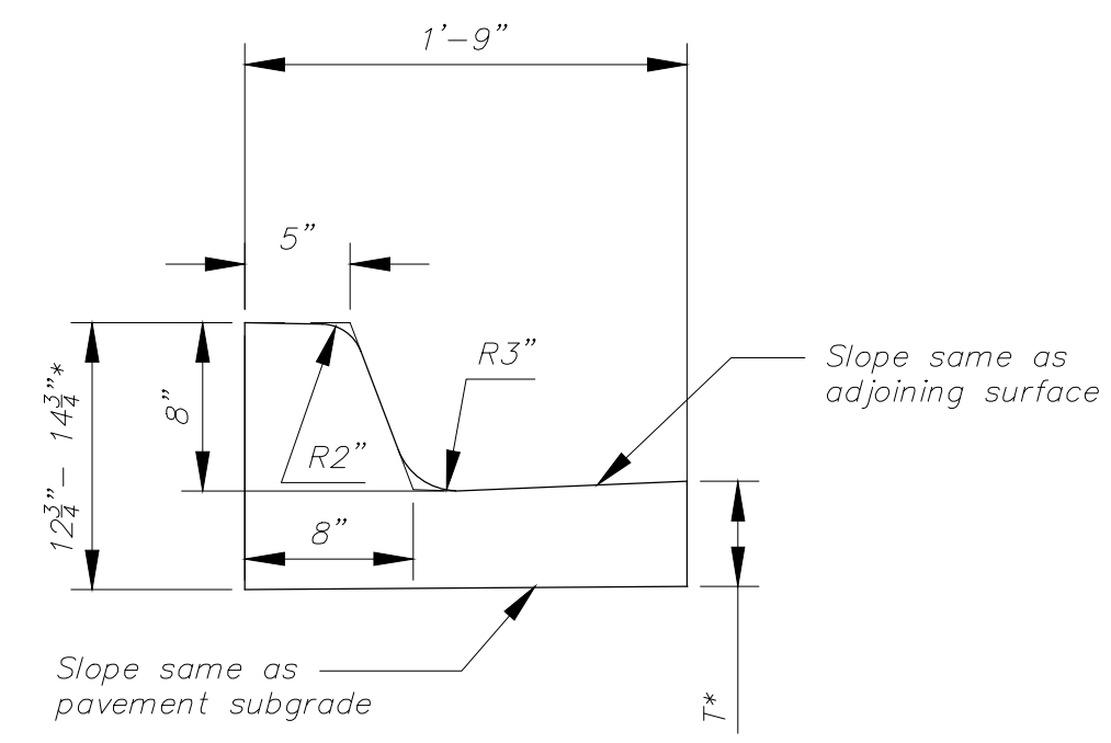
Combined Curb & Gutter (8") High Edge
