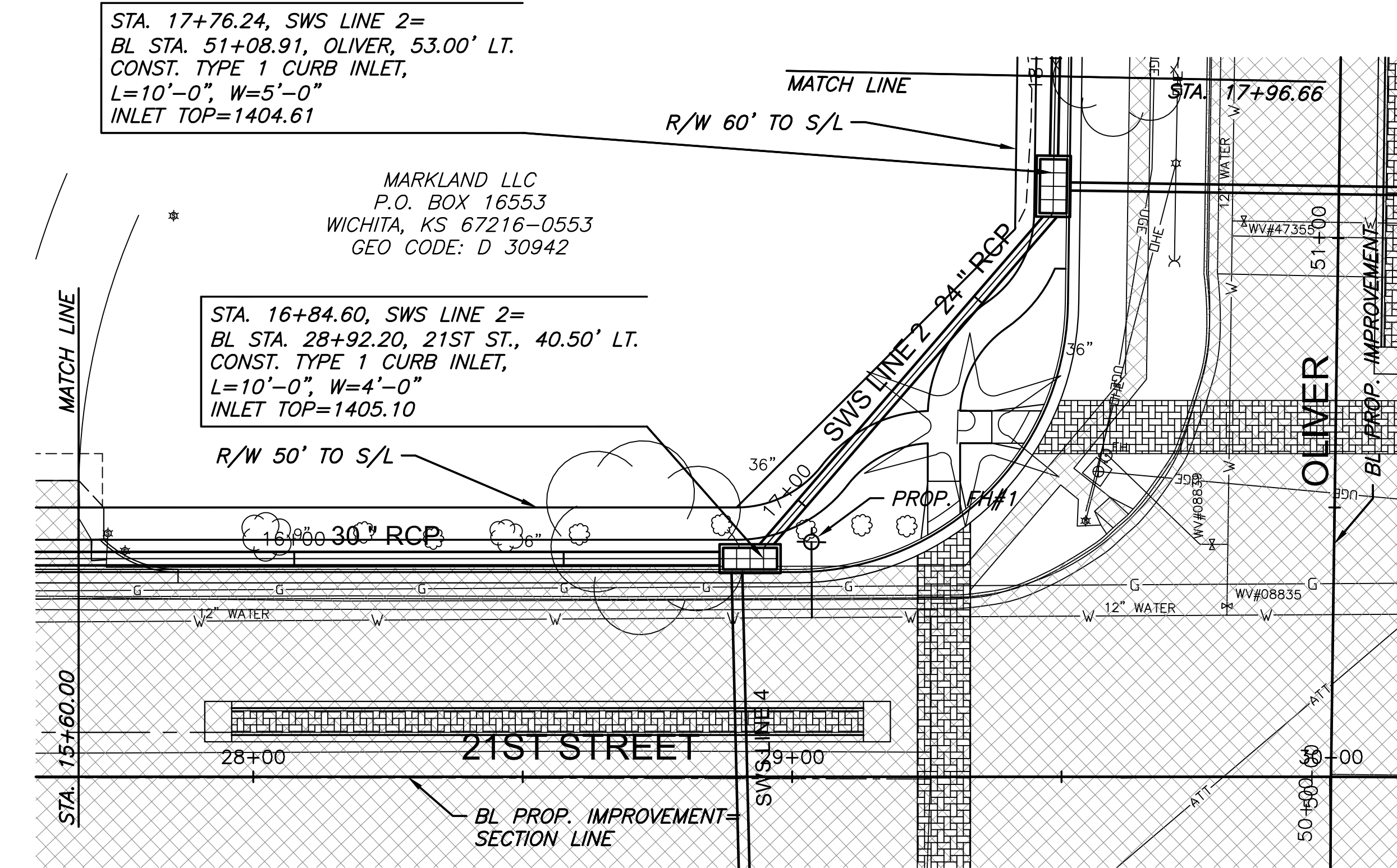
PLAN SWS LINE 2 CONT. PROFILE SWS LINE 2 CONT.
