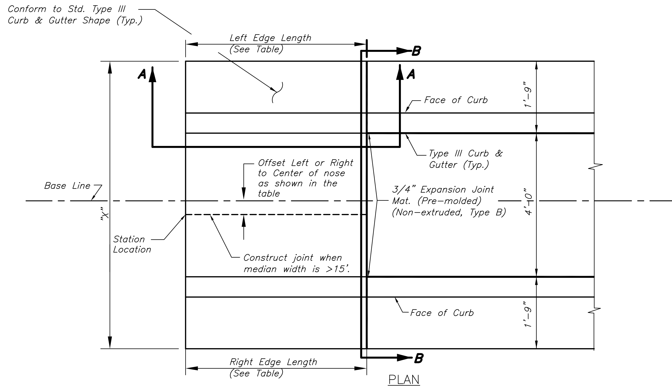
CONCRETE MEDIAN NOSE
