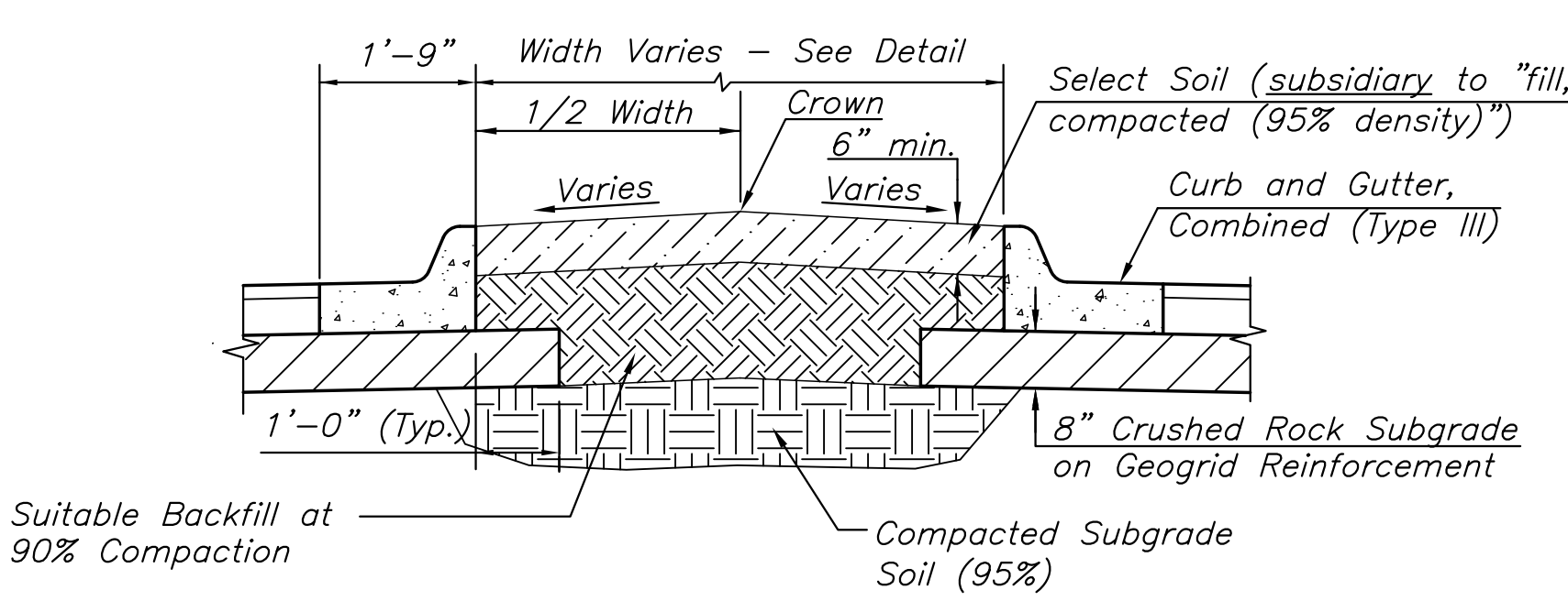
SELECT SOIL MEDIAN DETAIL
