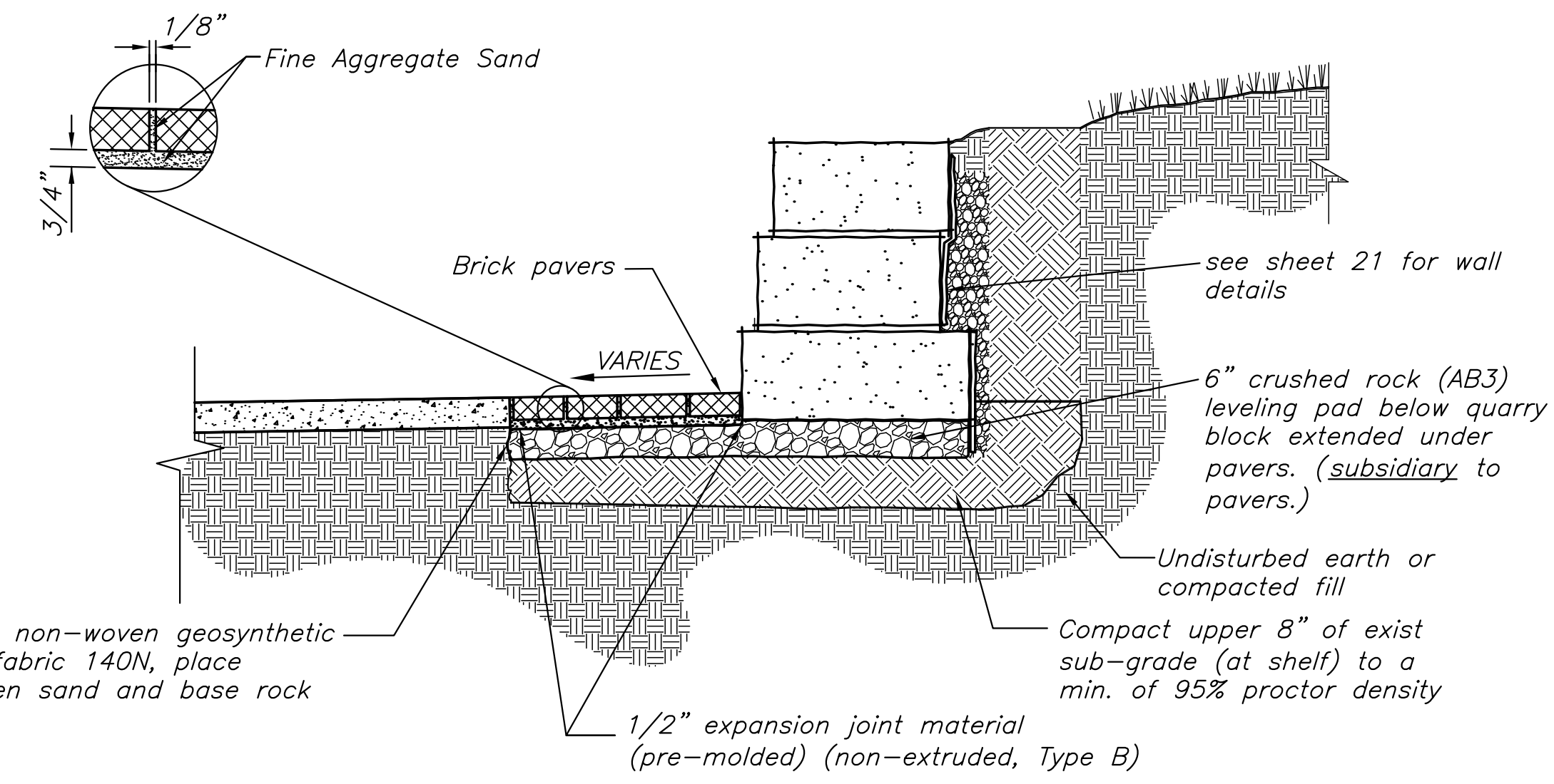
PAVING BRICK SIDEWALK DETAIL
