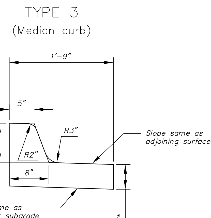
Combined Curb & Gutter (8")
