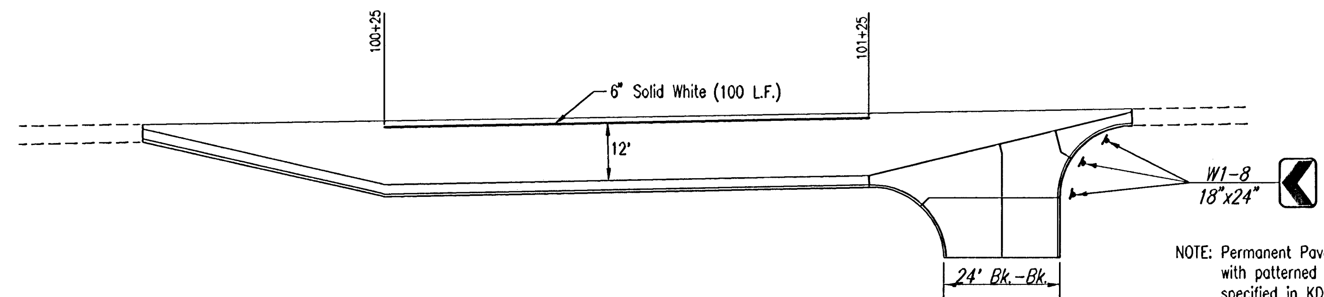
MARKING PLAN
