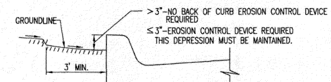
CURB BACKFILL DETAIL (STREET CONSTRUCTION ONLY)
