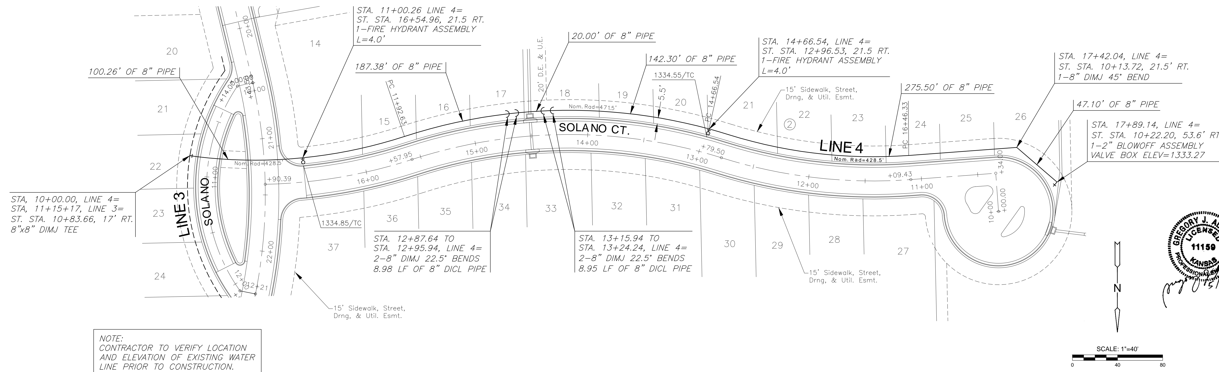
PLAN PH2 WTR LINE 4 PROFILE PH2 WTR LINE 4
