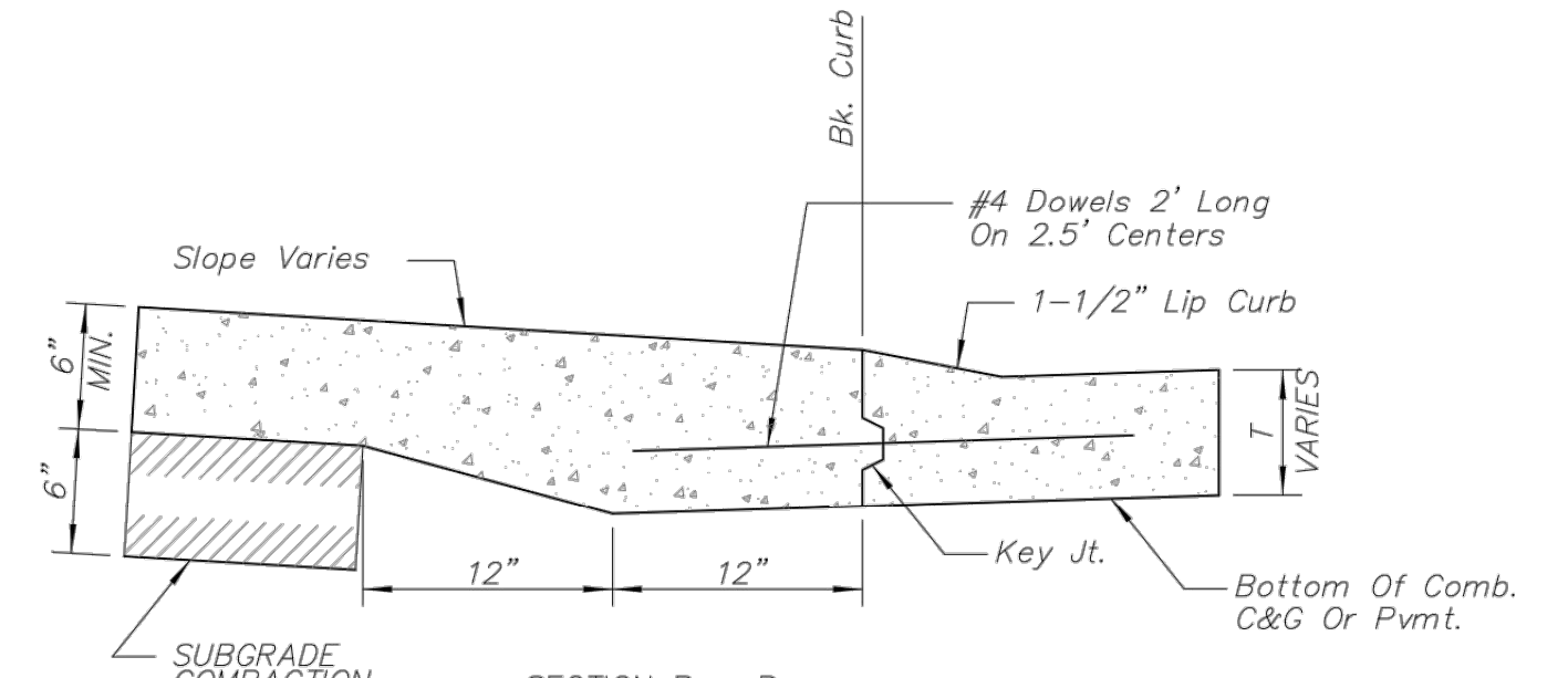
SECTION B - B BACK OF CURB DETAIL
