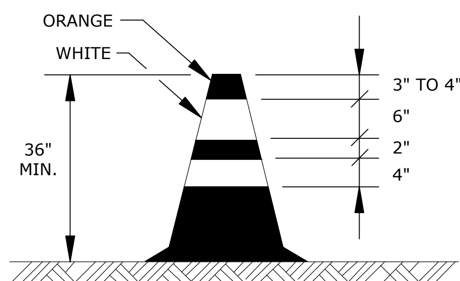
TRAFFIC CONE
