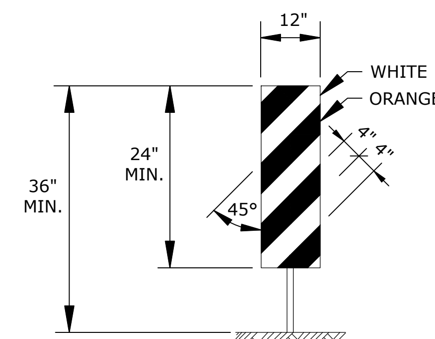
VERTICAL PANEL
