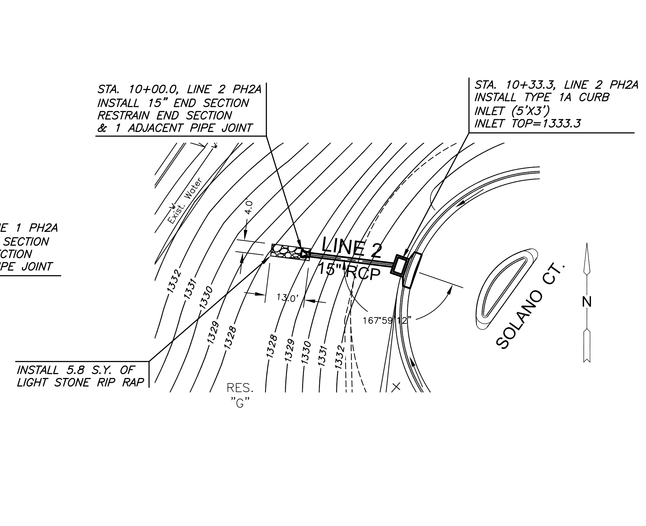
PLAN SWS LINE 2 PHASE 2A PROFILE SWS LINE 2 PHASE 2A
