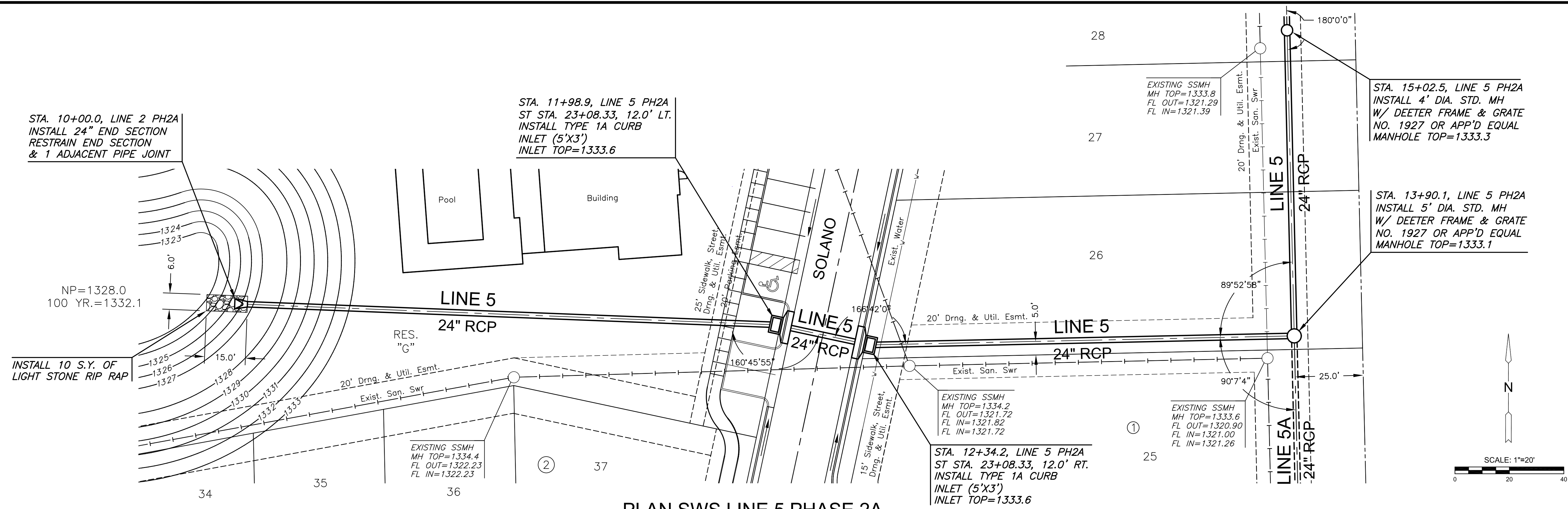
PLAN SWS LINE 5 PHASE 2A PROFILE SWS LINE 5 PHASE 2A
