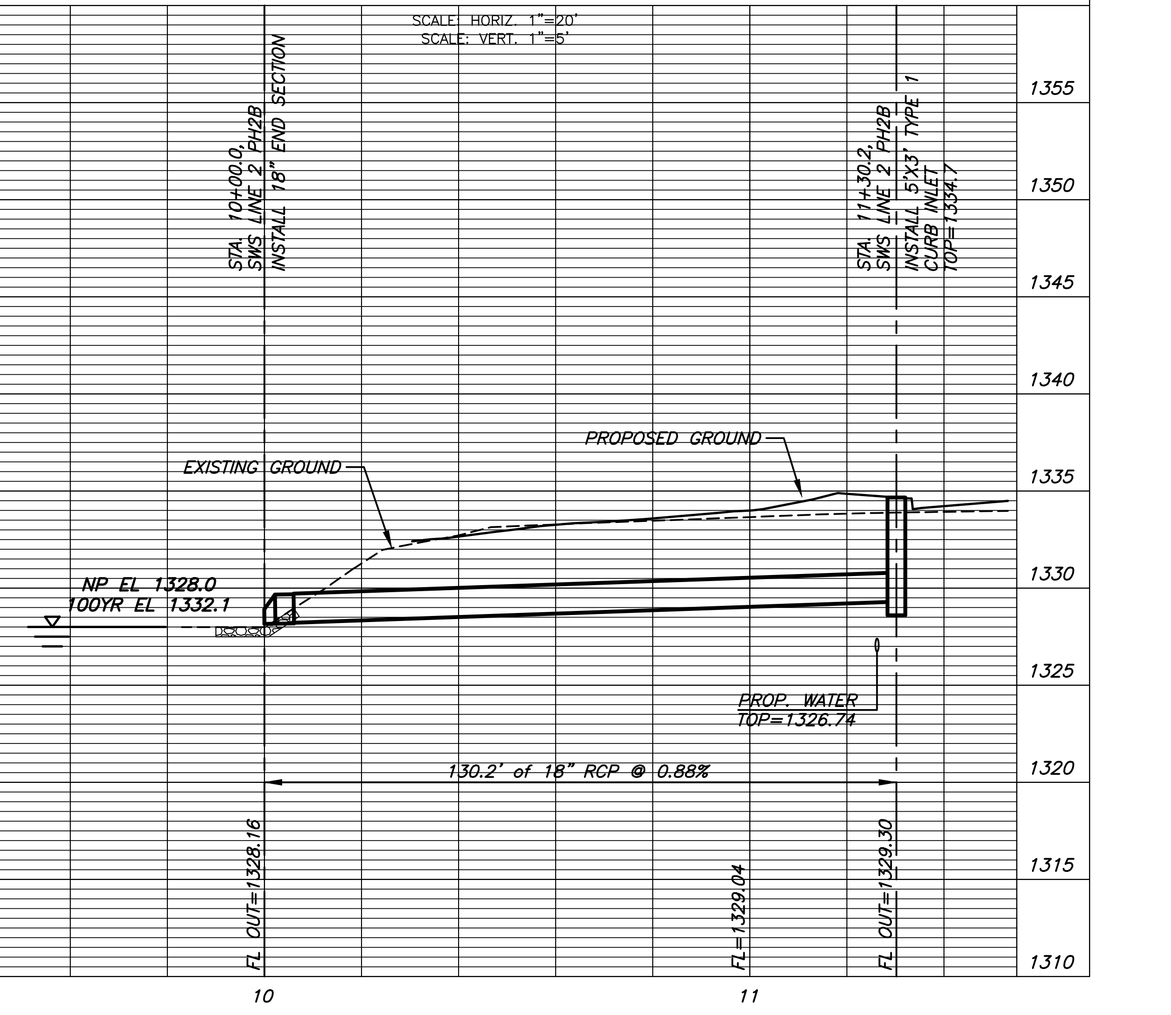
PROFILE SWS LINE 2 PHASE 2B
