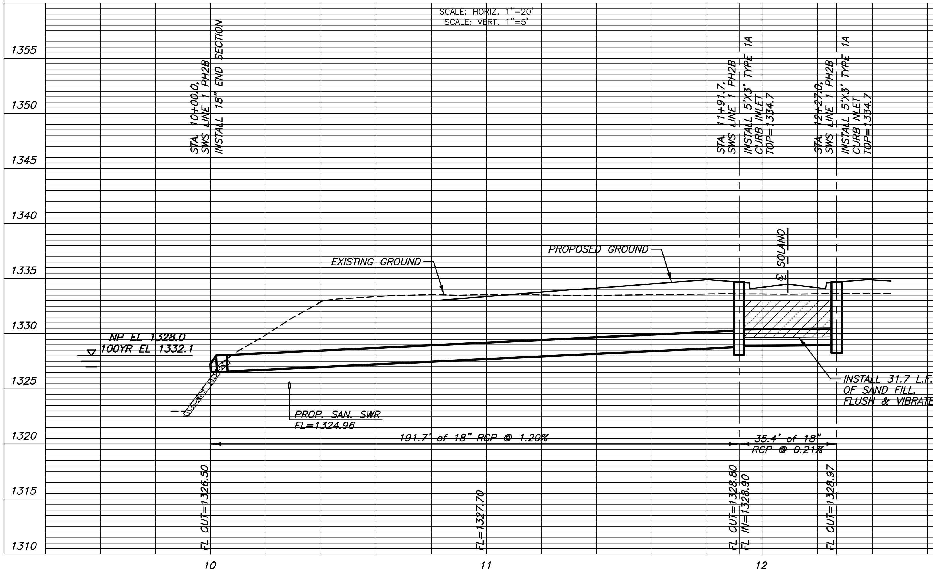
PROFILE SWS LINE 1 PHASE 2B
