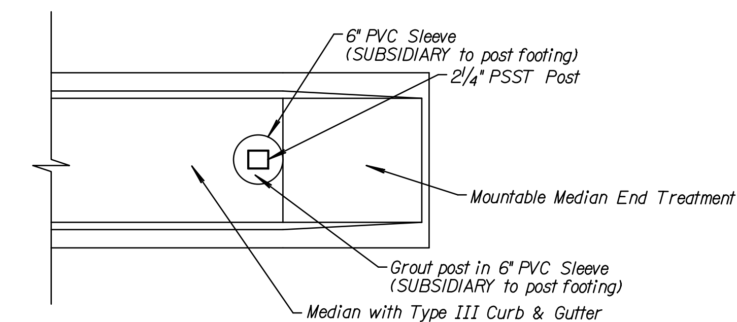
PSST POST BLOCK OUT DETAIL Not to Scale Block outs shall be used for all PSST Post located in the medians. The 6" pvc sleeves shall be installed prior to the placement of the Flowable Fill and 4" Concrete Pavement within the medians.
