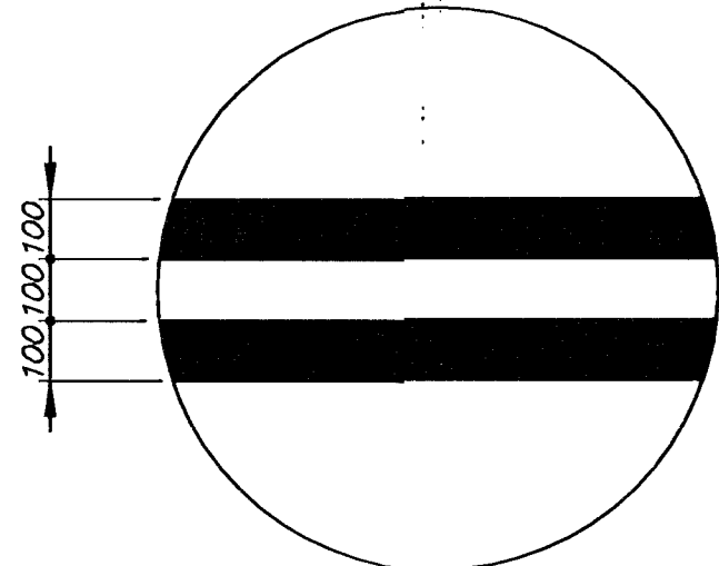
TYPICAL SPACING FOR DOUBLE YELLOW LINES
