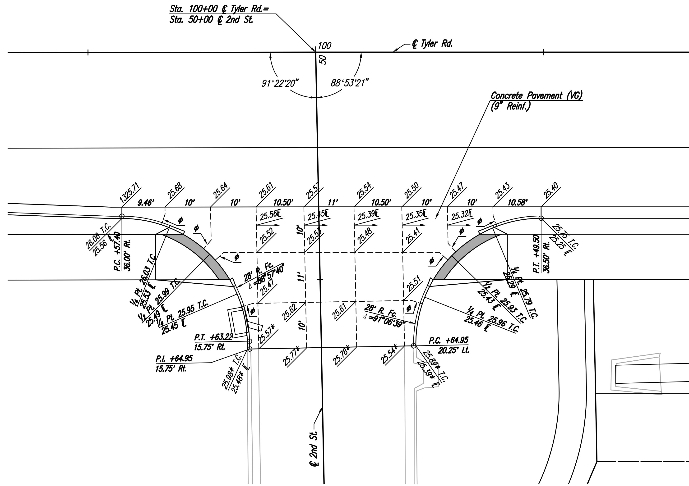
INTERSECTION 2ND. ST.
