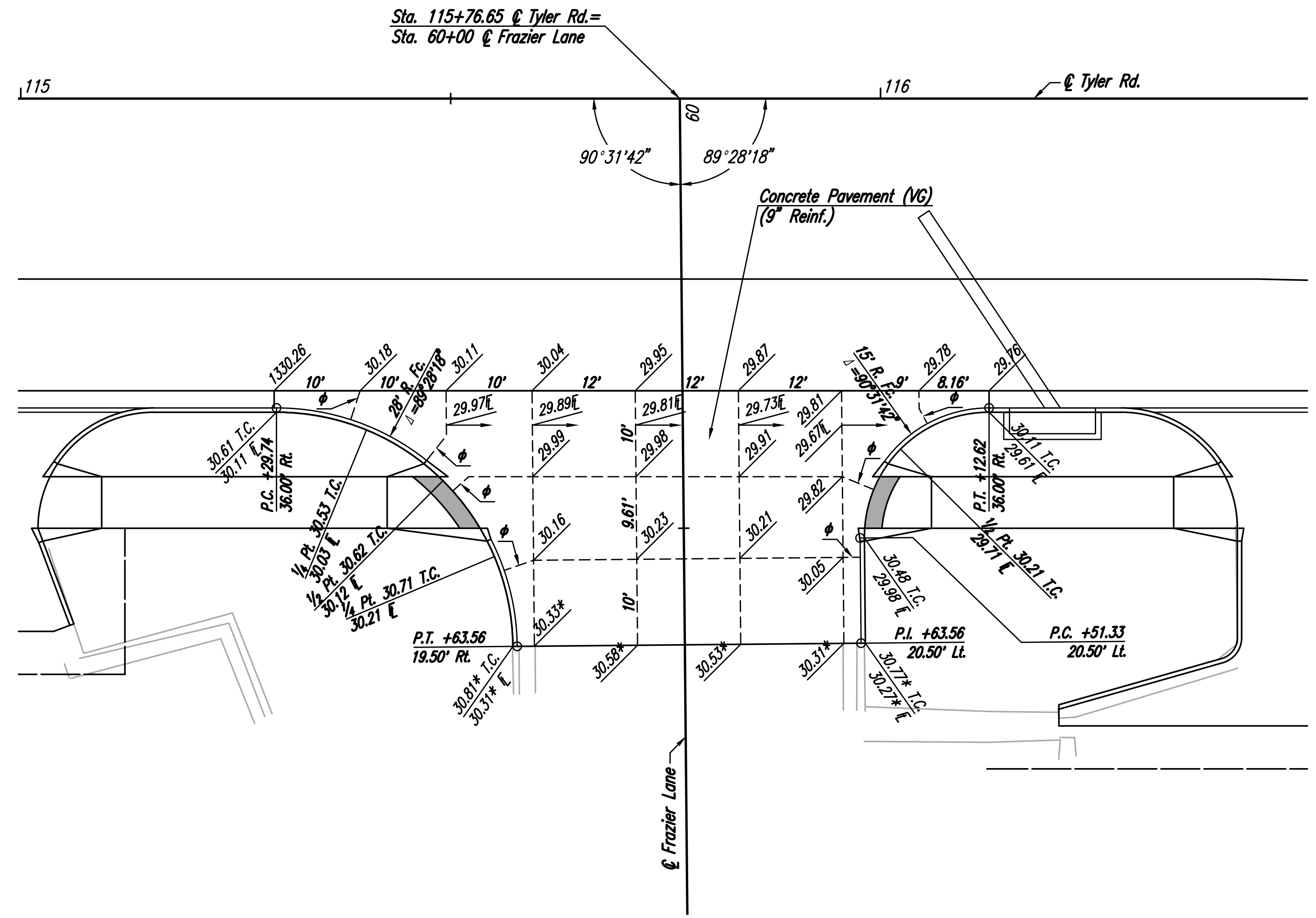
INTERSECTION FRAZIER LANE
