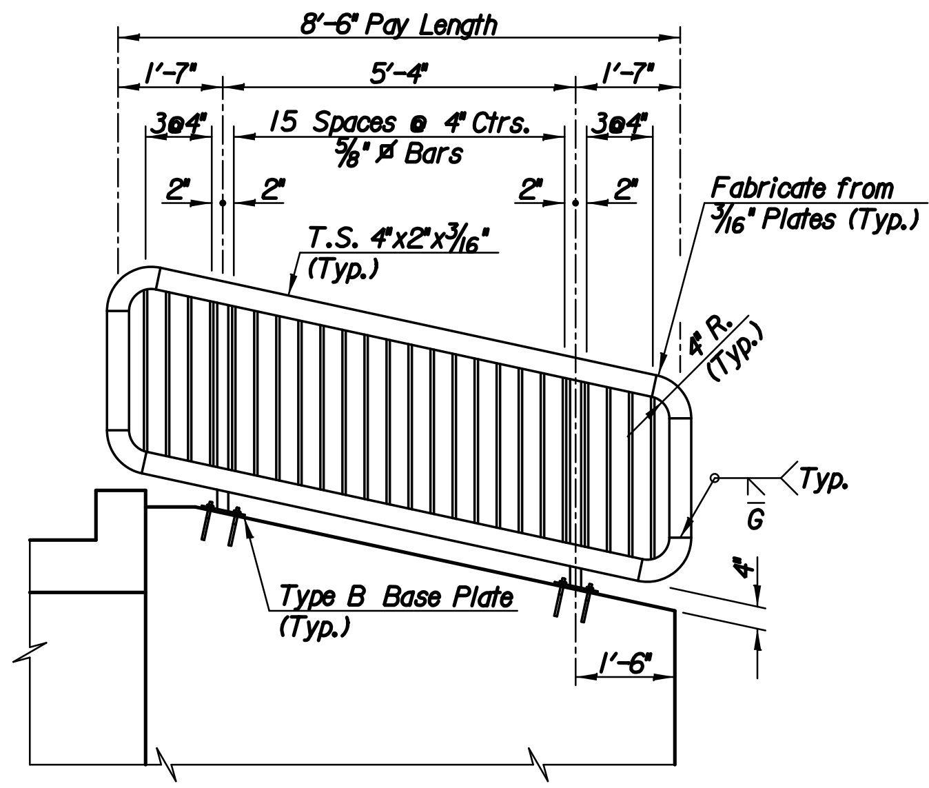
ELEVATION AT WINGWALL (2 Required)
