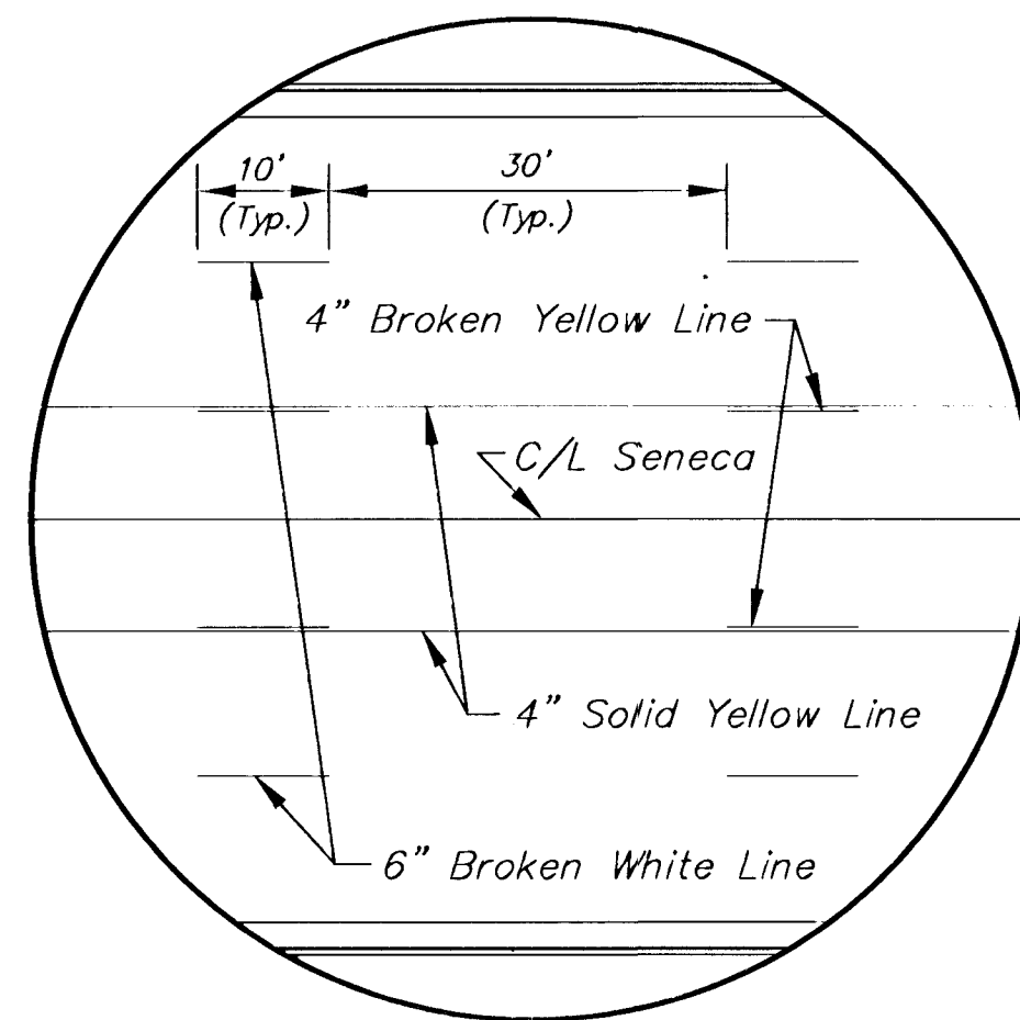
DETAIL "B"
