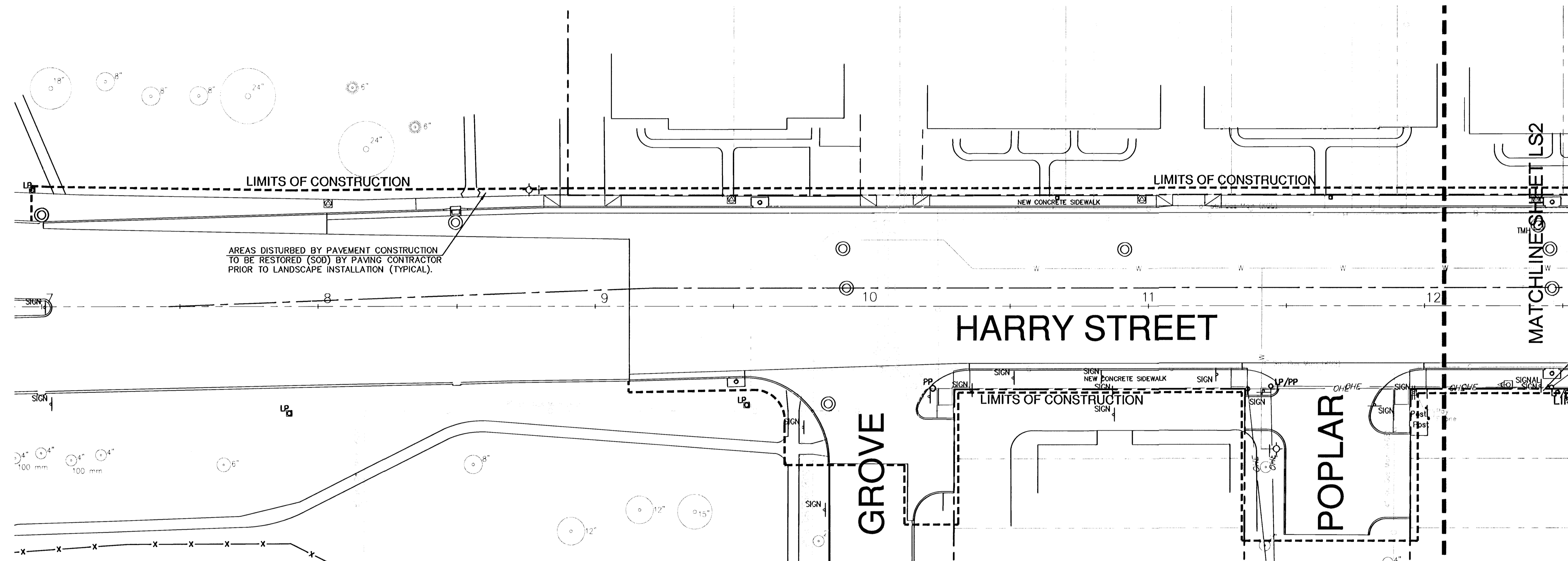
STREET PLANTING PLAN SCALE: 1"=20'-0"
