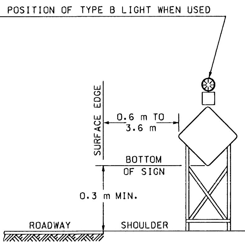
HEIGHT AND LATERAL DIMENSIONS FOR SIGNS MOUNTED ON SKIDS OR OTHER MOVABLE MOUNTS
