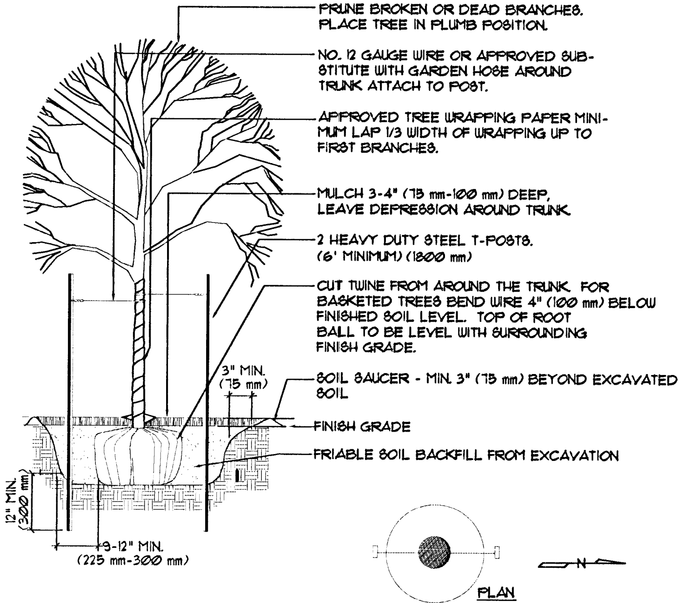
DECIDUOUS TREE PLANTING 2" (50 mm) CALIPER AND LARGER
