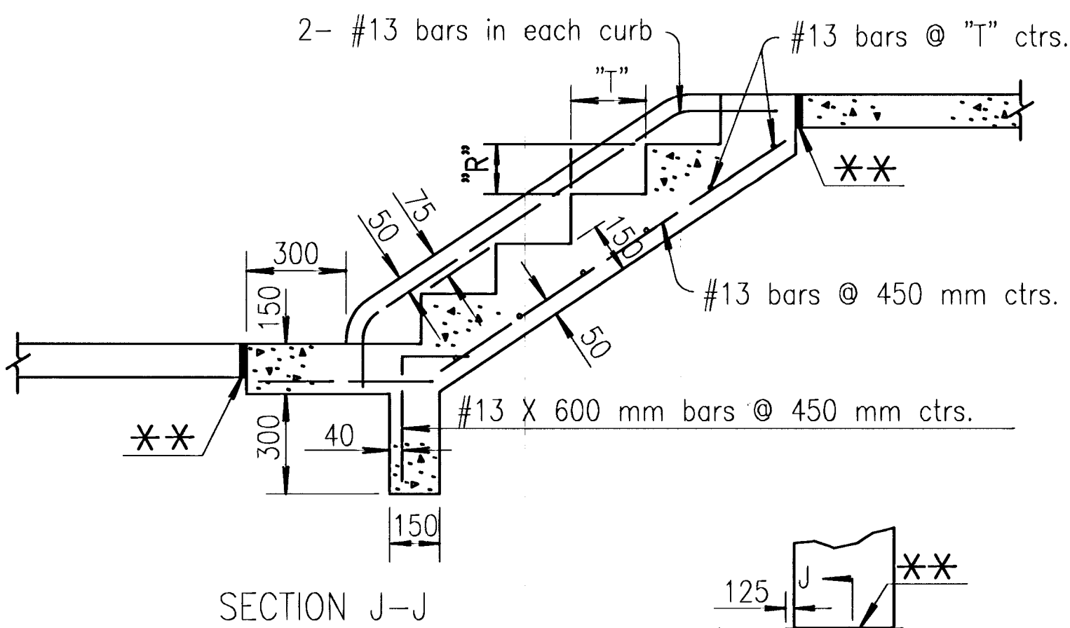
SECTION J-J
