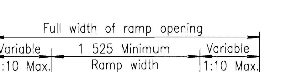
SECTION I-I
