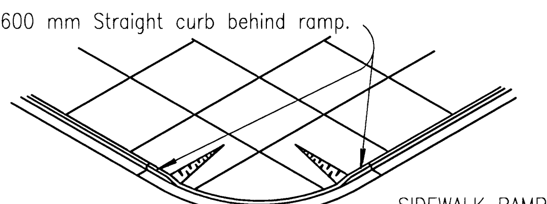
SIDEWALK RAMP TYPE 3
