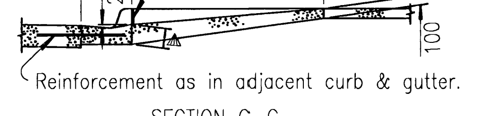
SECTION H-H
