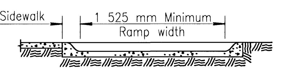
SECTION E-E
