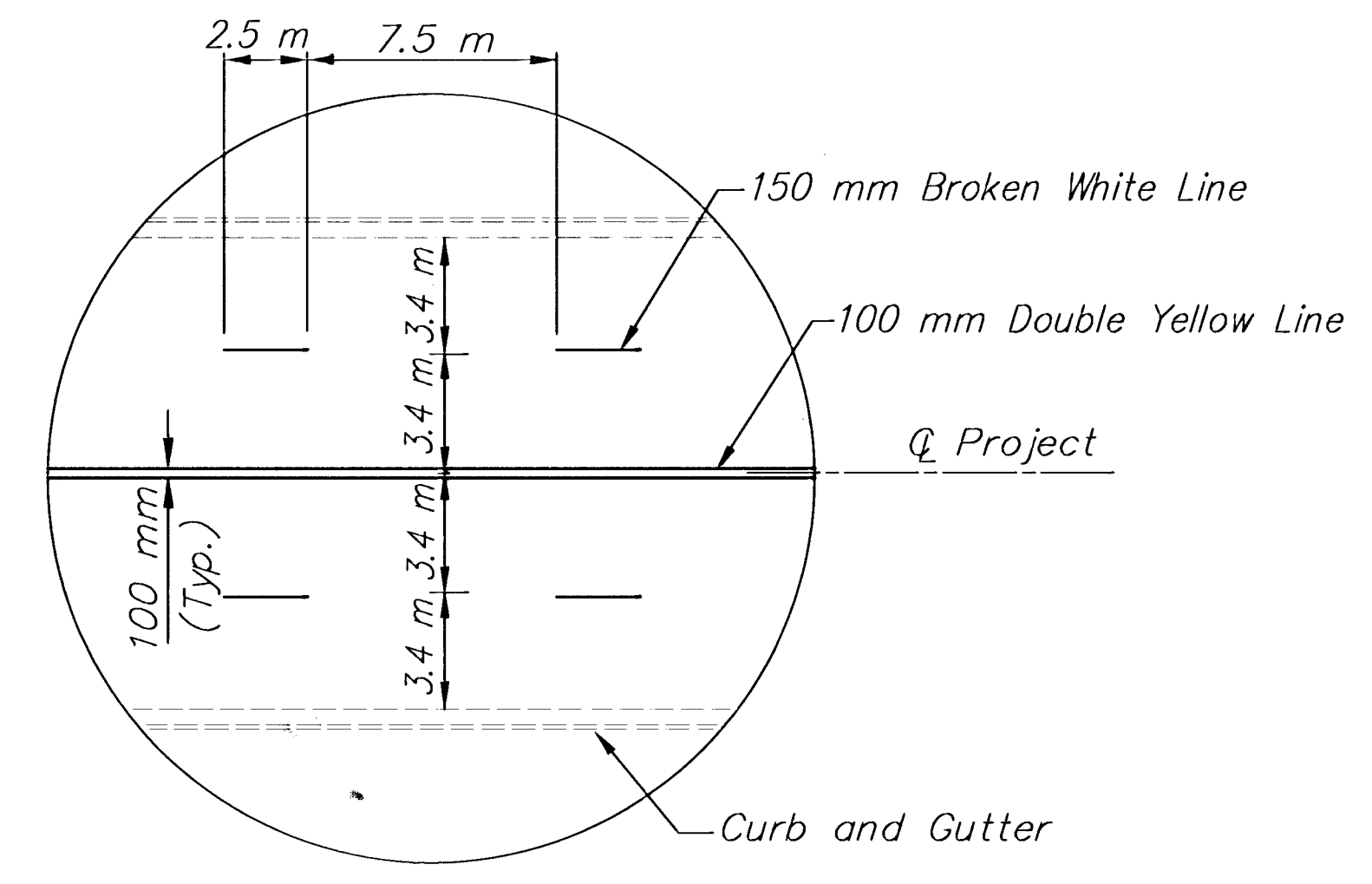
TYPICAL LANE DETAIL
