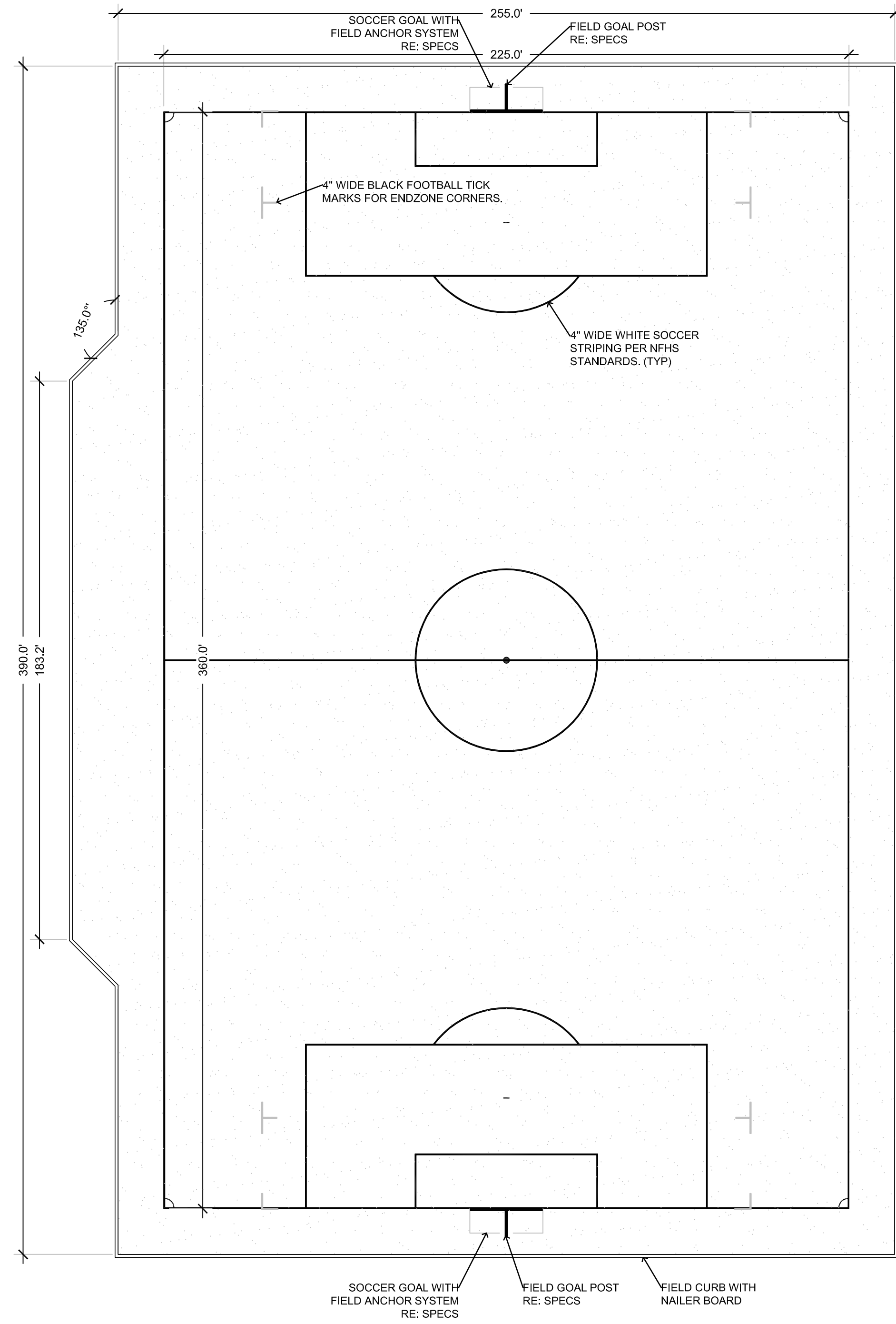
LAYOUT PLAN
