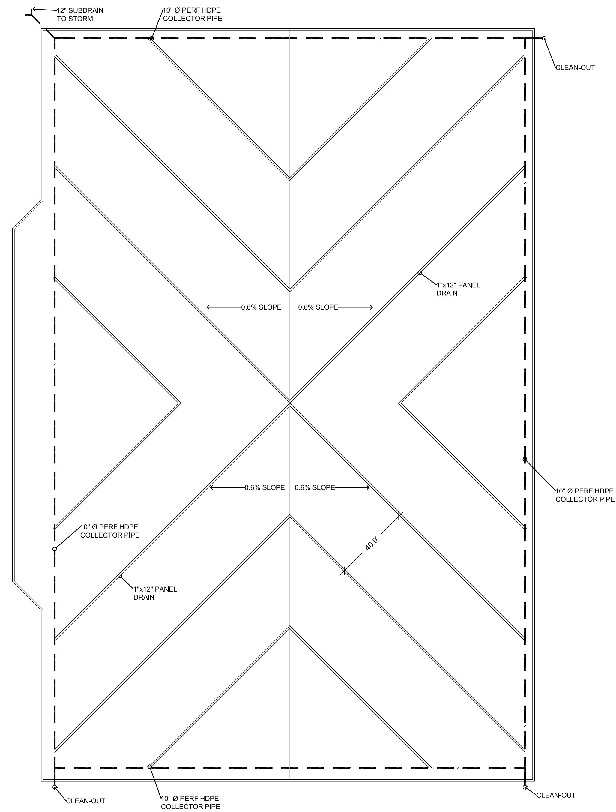
DRAINAGE PLAN
